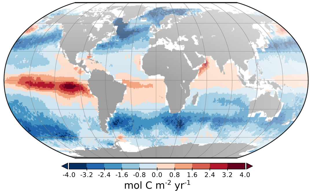
Figure 1. Illustrative map of annual \text{CO}_2 flux in 2010. Upward fluxes are defined as positive. Details are described in the main text.
