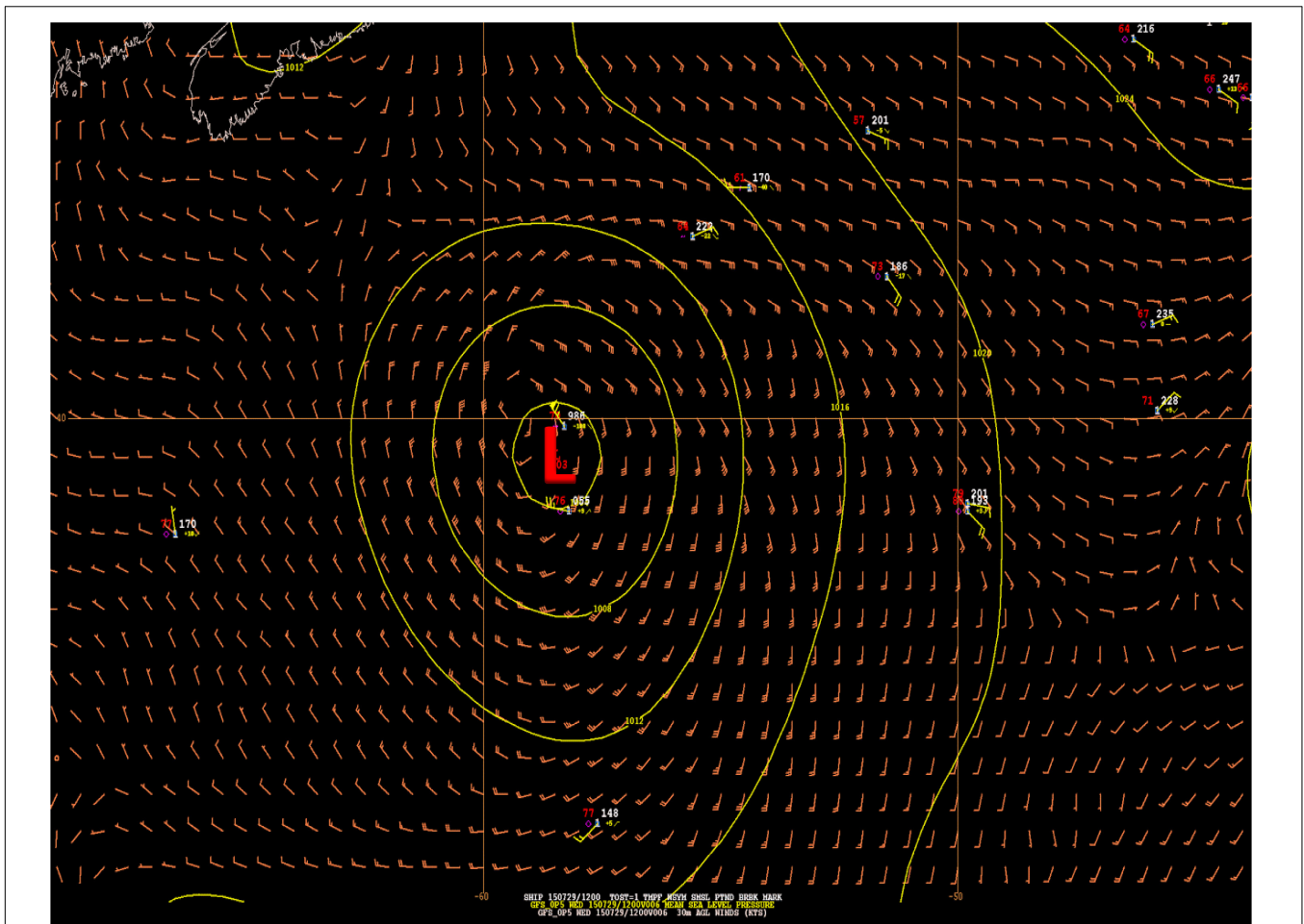
FIGURE 3 | GFS model 29 July 2015 0600 UTC 6-h forecast, valid 1200 UTC 29 July 2015, with available ship observations using standard synoptic station notation. Isobars are drawn with yellow lines, and the model wind field is indicated by wind barbs in orange. The low pressure center is located near 39°N, 58.5°W. Courtesy of National Oceanic and Atmospheric Administration, National Weather Service, Ocean Prediction Center.
