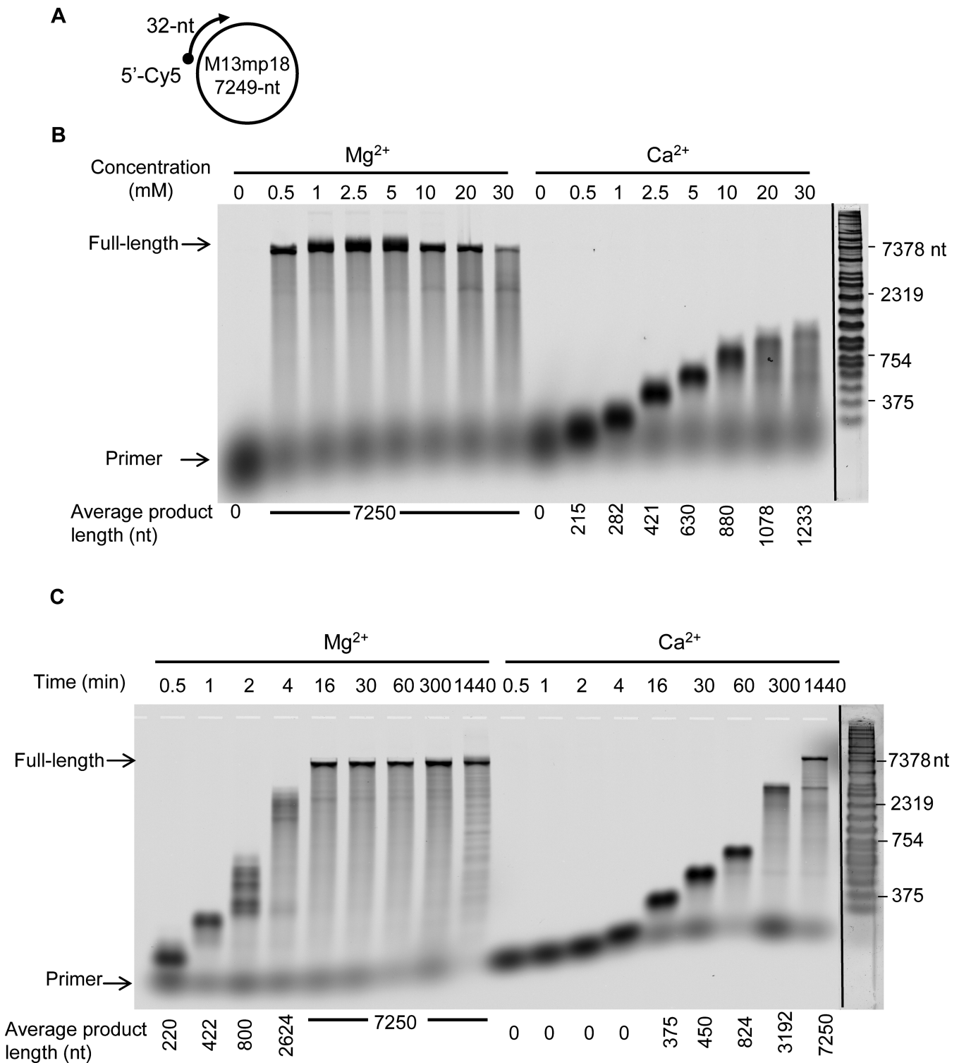
Figure 2. Modulation of DNA polymerization PabPolB with Mg^{2+} or Ca^{2+} on primed-M13mp18 DNA template. (A) Structure of the primer-template mimic, consisting of a Cy5-labeled 32-mer primer annealed to the circular M13mp18 DNA template of 7249-nt in length. (B) Extension of the primed-M13mp18 DNA template at the indicated Mg^{2+} or Ca^{2+} concentrations. The starting primer (32-nt) and full-length product (7249-nt) are shown arrowed on the left. Product length is indicated under the gel lanes. (C) Extension of the primed-M13mp18 DNA template for the times shown above the gels (min) at fixed Mg^{2+} or Ca^{2+} concentrations (5 mM). The starting primer (32-nt) and full-length product (7249-nt) are shown arrowed on the left. Product length is indicated under the gel lanes.
