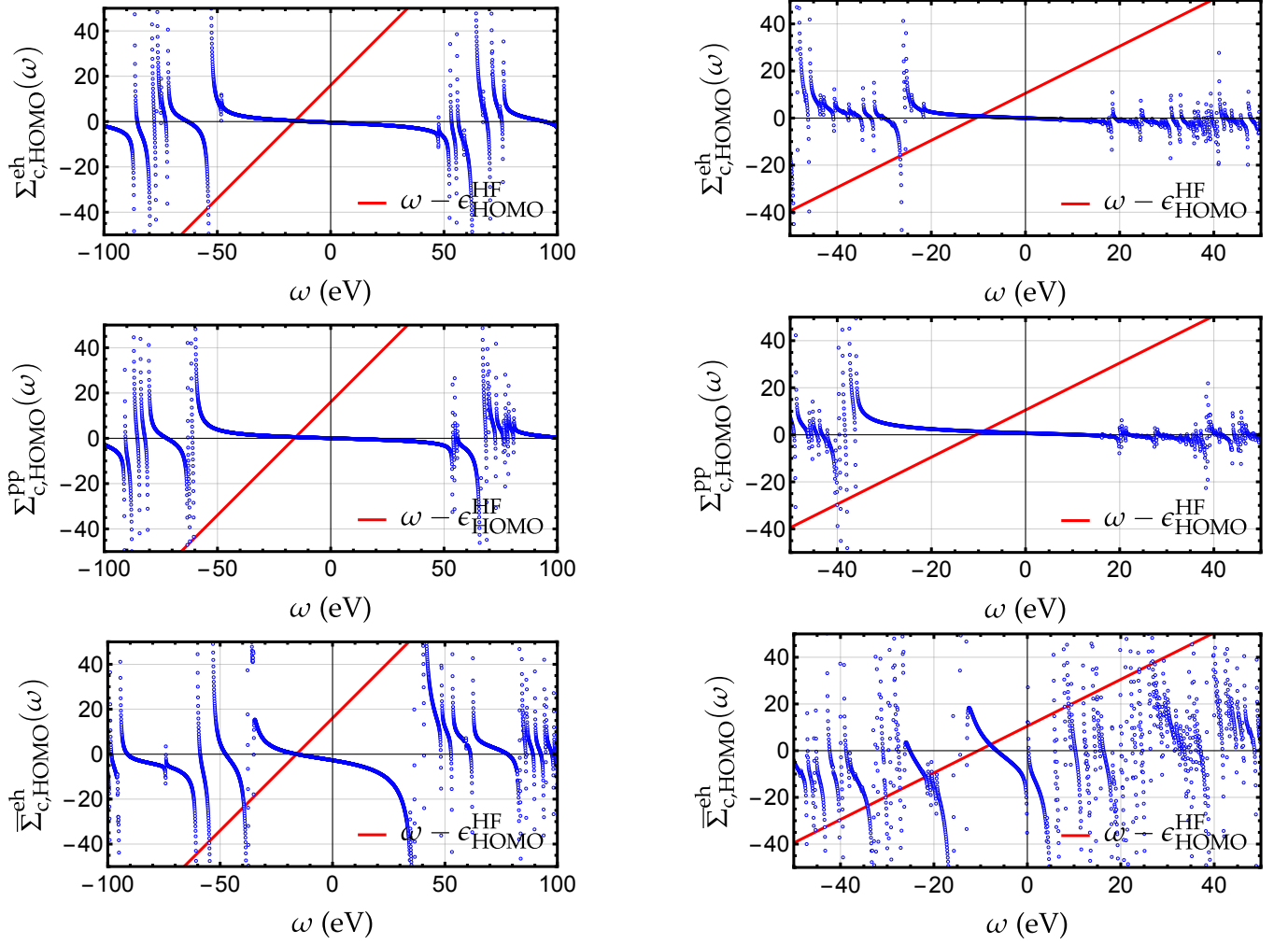
FIG. 5. Self-energy (blue curves) associated with the HOMO orbital of Ar (left) and BeO (right) computed at the G_0W_0 (top), G_0T_0^{pp} (middle), and G_0T_0^{eh} (bottom) levels with the def2-TVZPP basis. The solutions of the quasiparticle equation are given by the intersection of the blue and red curves. Raw data can be found in supplementary material .
