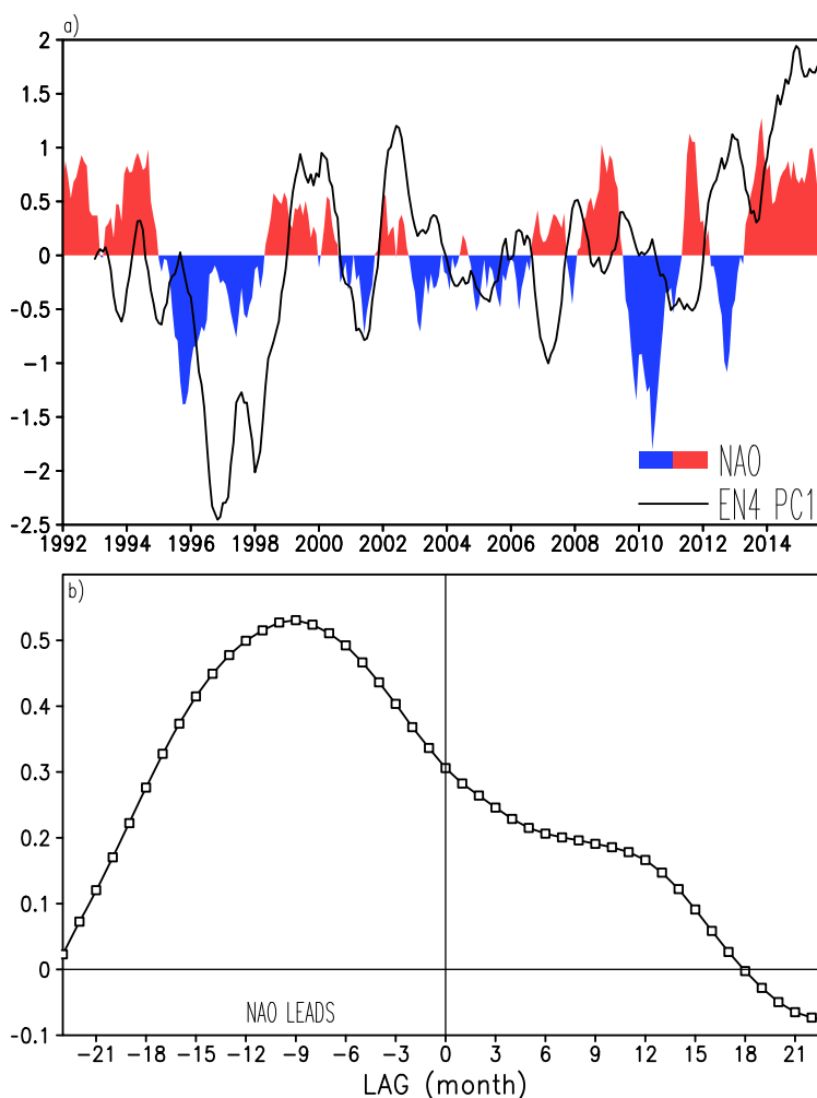
Figure 5. (a) Time series of annually smoothed station-based NAO index [Hurrell et al., 2003] and the leading principal component (PC1) of the EN4 analysis SST, SSS, and SSH (from Figure 4g). (b) Lagged correlation between NAO and PC1.
