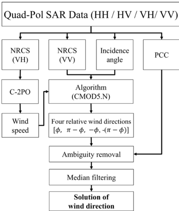
Fig. 5. Schematic flow chart of the wind retrieval from quad-polarization SAR data, where the acronyms indicate the normalized radar cross section (NRCS), polarization correlation coefficient (PCC), C-band cross-polarized ocean backscatter model (C-2PO), and C-band geophysical model function for the equivalent neutral wind (CMOD5.N), respectively.
