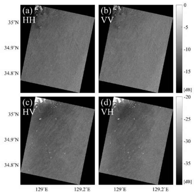
Fig. 4. Distributions of the normalized radar cross-section (dB) at (a) HH-, (b) VV-, (c) HV-, and (d) VH-polarization state.
