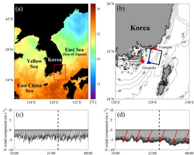
Fig. 3. (a) Distribution of daily mean sea surface temperature (SST, °C) from the Multi-scale Ultra-high Resolution (MUR) SST data on August 23, 2008 in the seas around the Korean Peninsula, where the red box and black box indicate the study area and the location of the Radarsat-2 image, and (b) an enlarged image of the bathymetry contour in the study area, where the blue triangle and red circles indicate the locations of the Korean Meteorological Administration (KMA) buoy station (ID: Geoje-do, 128.90°E, 34.76°N) and Automatic Weather Stations (AWSs), respectively. Time-series of wind vectors from the AWS measurements at (c) Youngdo (129.06°E, 35.06°N) and (d) Seoimal (128.73°E, 34.78°N), where dotted lines indicate the acquisition time of the Radarsat-2 image and red vectors indicate the hourly wind vectors from the in-situ buoy measurement.
