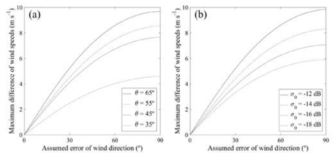
Fig. 2. Maximum differences in retrieved wind speeds from the CMOD5.N algorithm as a function of an error in wind direction. (a) for an NRCS value of -15 dB and (b) at the incidence angle value of 45^{\circ} .
