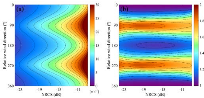
Fig. 1. Distributions of (a) estimated wind speeds ( \text{m s}^{-1} ) as a function of the NRCS (dB) and wind direction ( ^{\circ} ) at a given incidence angle ( 45^{\circ} ) using the CMOD5.N algorithm and (b) ratios of wind speeds divided by the minimum value of wind speed for a given value.
