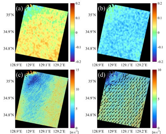
Fig. 6. (a) Real and (b) imaginary parts of the polarization correlation coefficients (PCC) from the Radarsat-2 image. Distributions of (c) wind speed ( \text{m s}^{-1} ) from VH-polarized SAR data using the C-2PO algorithm and (d) the retrieved wind fields from the PCC and CMOD5.N algorithm after median filtering.
