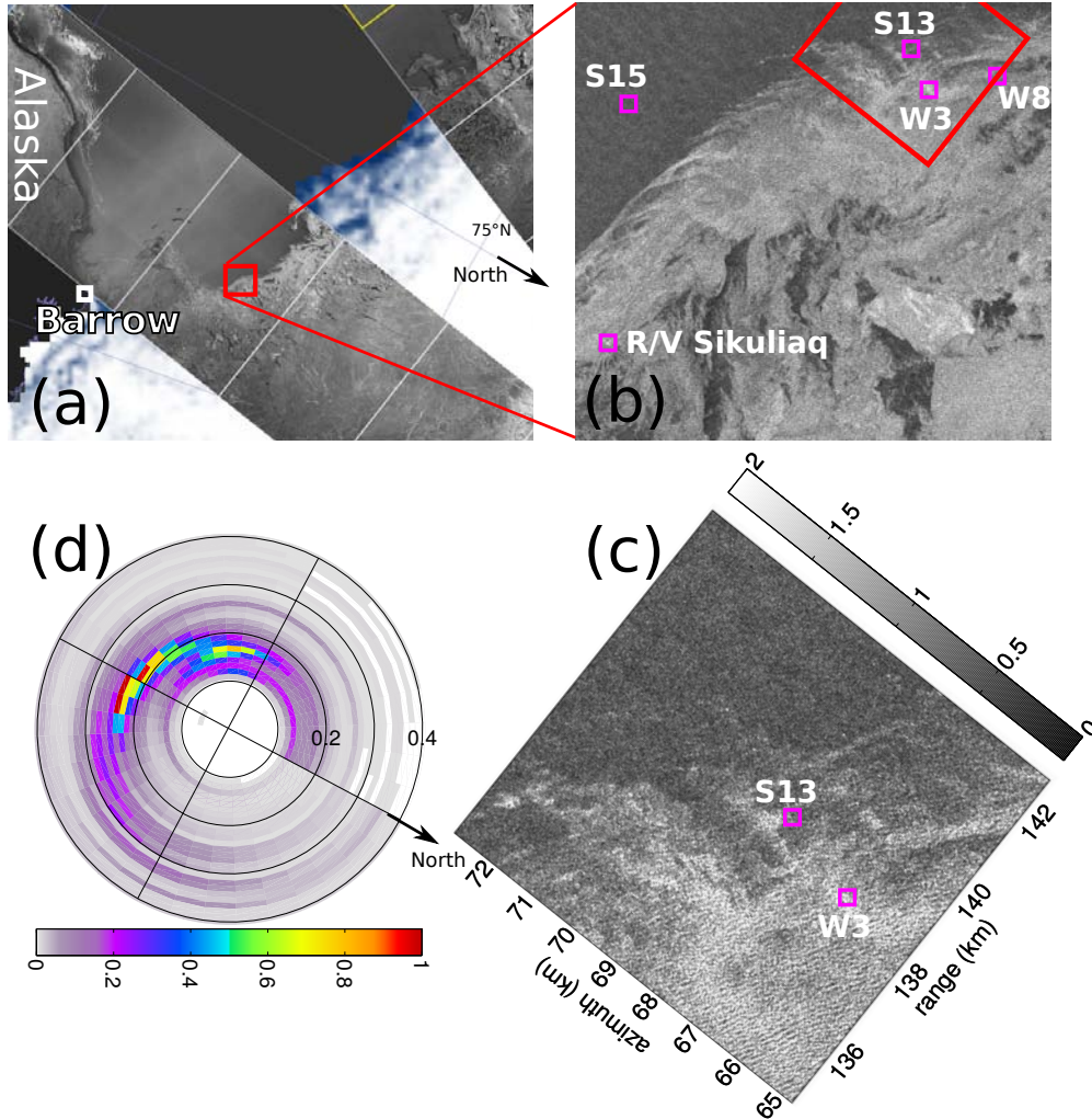
Figure 11: Context of the S1A IW image acquired on November 1st, 2015, at 17:23 UTC, and available in situ data. The full image at full resolution can be viewed at http://bit.ly/22JFruo . (a) SAR-derived roughness (gray scale) showing open water between the Alaska shoreline, to the West of Barrow, and the measurement locations in the red box. (b) Location of the R/V Sikuliaq and some of the measurement buoys. Note that buoy S15 is in open water. (c) piece of the SAR image around the buoys S13 to W3. (d) Directional spectrum estimated from S15 data using the Maximum Entropy Method (Lygre and Krogstad, 1986).
