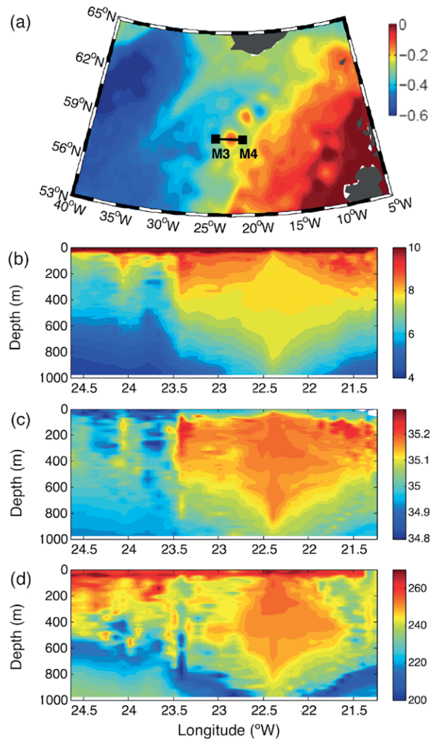
FIG. 9. (a) ADT (m) between 23 Jul and 2 Aug 2015, showing an anticyclonic eddy on the OSNAP line. The two black squares denote moorings M3 and M4, and a black line represents the sampling path. (b) Temperature (°C), (c) salinity, and (d) dissolved oxygen ( \mu\text{mol kg}^{-1} ) data recorded by the glider during the eddy scenario are shown.
