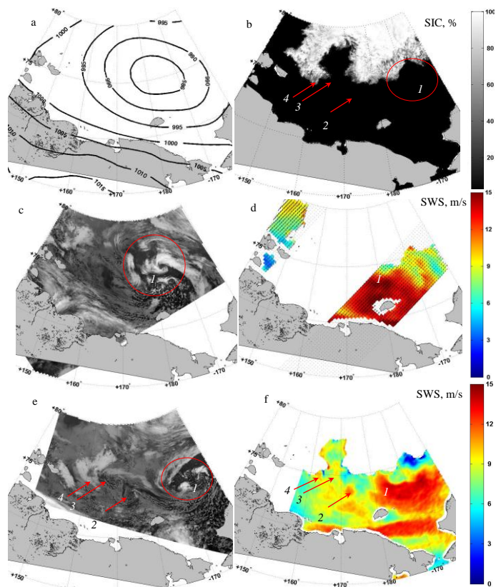
Fig. 3. A system of polar lows over the East Siberian Sea on 2015, 29 September: (a) ERA-Interim MSLP, 00:00 UTC; (b) AMSR2 SIC (%); (c) Aqua MODIS IR image at ~ 00:15 UTC; (d) MetOp-B ASCAT SWS (m/s) at ~ 00:50 UTC; (e) Aqua MODIS infrared image at ~ 15:10 UTC; (f) GCOM-W1 AMSR2 SWS (m/s) at ~ 15:10 UTC.
