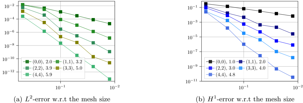
Figure 3: Same setting as in Figure 2, but for an analytical solution with nonzero initial and boundary conditions.
