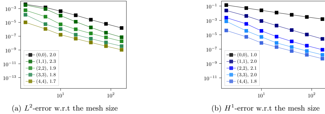
Figure 1: Convergence of the L^2 - and H^1 -errors at the final time as a function of the mesh size, polynomial orders k \in \{0, 1, 2, 3, 4\} , equal-order setting, \mathfrak{T} = 0.2 , \Delta t = 0.8\eta(k)\mu^{-1}h .
