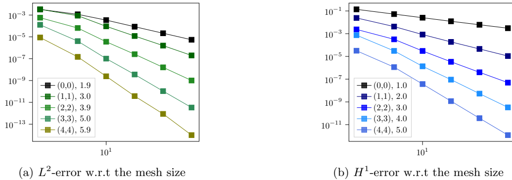
Figure 2: Convergence of the L^2 - and H^1 -errors at the final time as a function of the mesh size, polynomial orders k \in \{0, 1, 2, 3, 4\} , equal-order setting, \mathfrak{T} = 0.2 , \Delta t \ll h .
