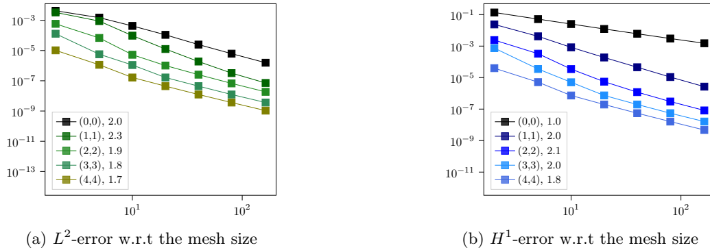
Figure 1: Convergence of the L^2 - and H^1 -errors at the final time as a function of the mesh size, polynomial orders k \in \{0, 1, 2, 3, 4\} , equal-order setting, \varpi = 0.2 , \Delta t = 0.8\eta\mu^{-1}h .
