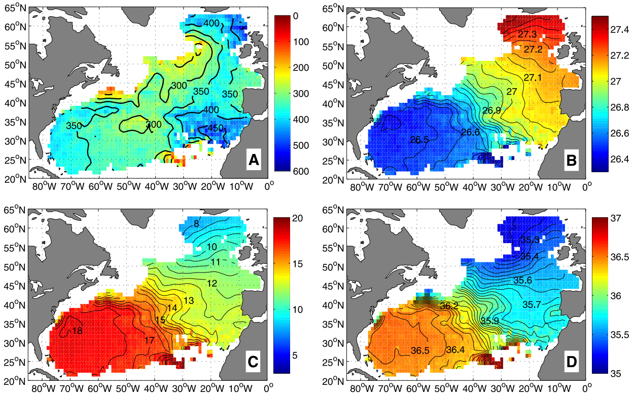
FIG. B1. Properties of the surface mode waters identified by OAC-P as overlying the pycnocline. (a) Depth with contours every 50 m. (b) Term \sigma_0 with contours every 0.05 \text{kg m}^{-3} . (c) Temperature with contours every 0.5°C. (d) Salinity with contours every 0.05.
