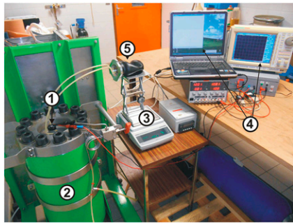
FIG. 6. (left) Hydraulic test bench used for the assessment of the pump efficiency. Hydraulic end cap under test (1). Hyperbaric test tank (2). Scales to weigh the oil transfers during pump or valve activations (3). Computers and oscilloscope for monitoring and control (4). Oil reservoir (5). (right) Current absorbed by the pump during oil transfers.
