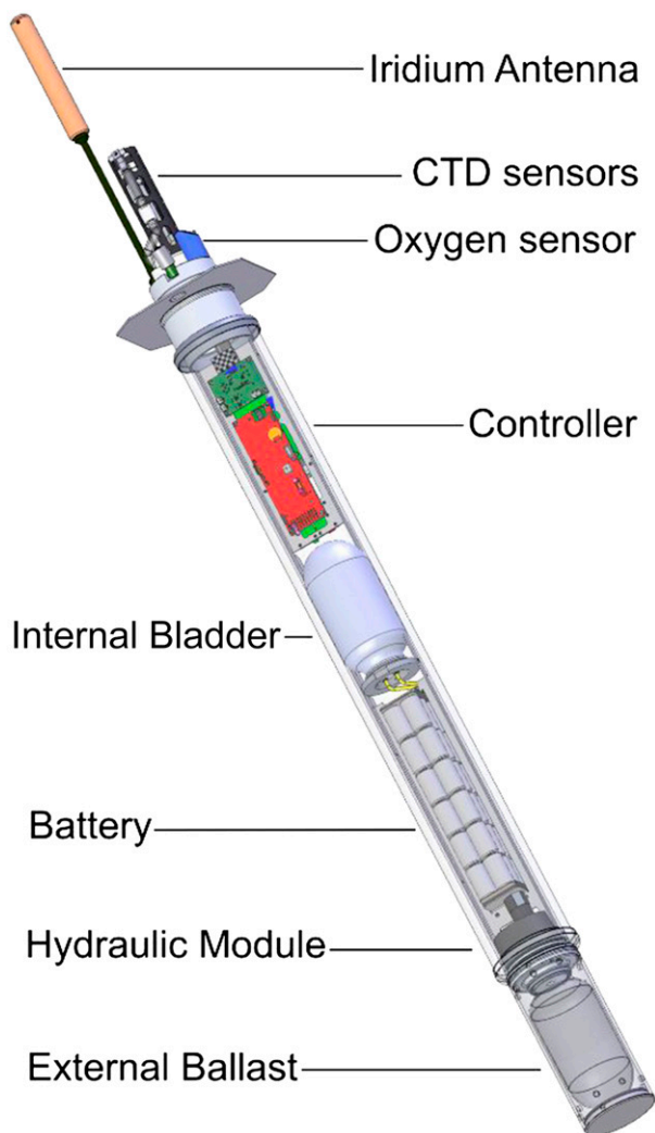
FIG. 3. Deep-Arvor 3D with subsets. This exploded view shows the main subassemblies of the float.
