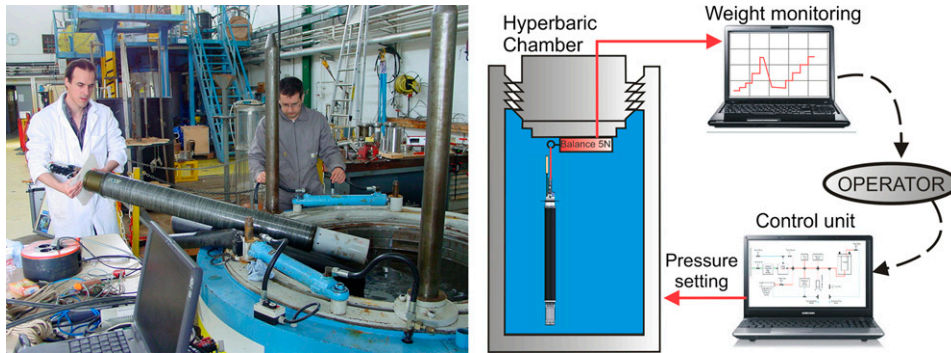
FIG. 9. Operational mission in pressure tank. The float is suspended in a hyperbaric tank and its weight is measured by a balance. The operator takes this weight into account and controls the pressure set point of the tank. Thus, a whole mission can be performed in realistic conditions.
