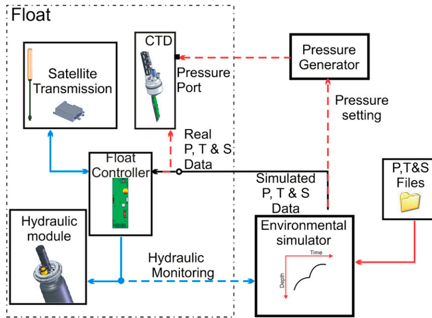
FIG. 8. Environmental test bench for the embedded software. The float part (surrounded by a dashed black line) is in operational mode. The environmental simulator continuously monitors the activations of the float engine, and hence computes the pressure to be applied to it according to the laws of motion of the float. Thus, a whole mission can be performed in a simulated environmental situation.
