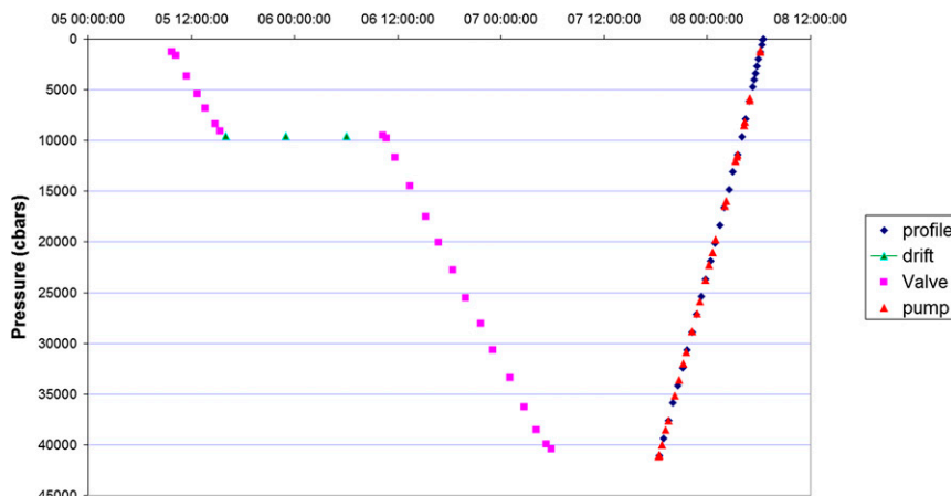
FIG. 5. Technical data sent by the float. Actions carried out by the engine are mentioned with the pink square and red triangle signs. The green triangle represents the measurements done during drift at parking depth. The blue lozenge sign represents measurements that are dated during profile.
