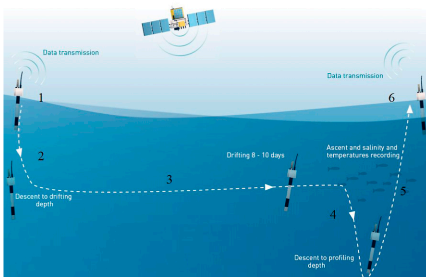
FIG. 1. Typical operational cycle of an Argo profiling float (courtesy of Euro-Argo Research Infrastructure). The float reduces its buoyancy (1), dives (2), and drifts at parking depth (3). Then it travels to the profile depth (4) and makes its measurement during the ascent (5). Transmissions and positioning are done at surface at the end of each cycle (6).
