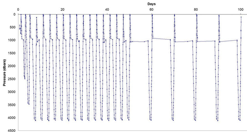
FIG. 12. Vertical behavior of the float. This partial figure illustrates the behavior of the float for the first 3 months and the effect of remote commands that are sent in order to modify its mission scheme.
