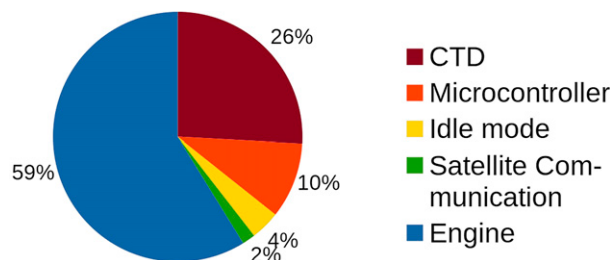
FIG. 4. Energy consumption pattern. The main power is used when the float moves in the water column (blue part). The power consumed when measuring represents a quarter of the total power, which is due to the continuous sampling and pumping of the CTD along the profile.
