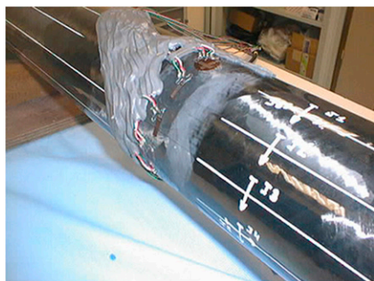
FIG. 7. Testing the tube in the pressure tank. (left) Before the test the tube is fitted with strain gauges stuck around the hull. (right) During the test deformations of the gauges are measured ( \mu strain) while pressure cycles are applied by the pressure tank for 3 days.
