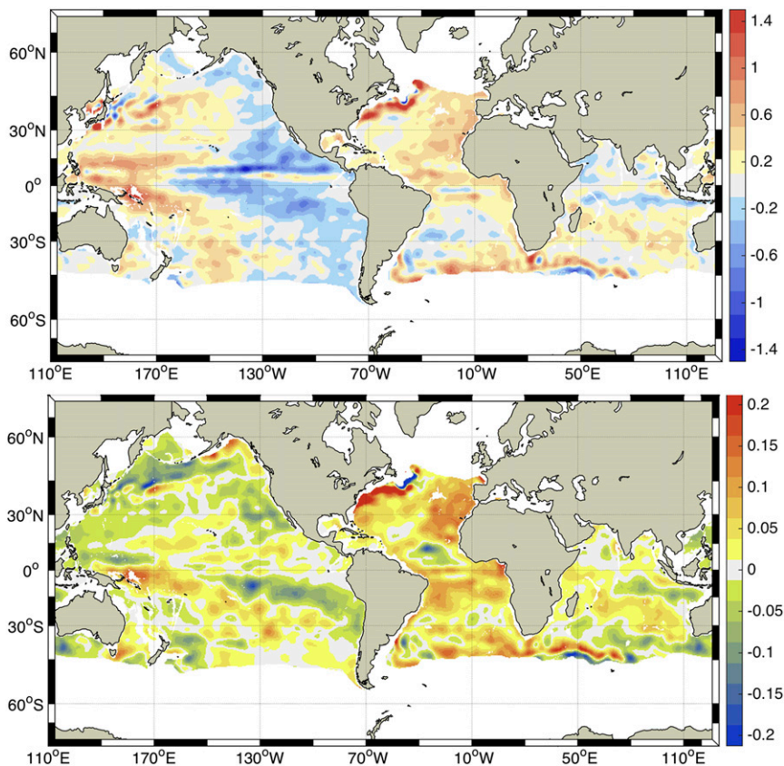
FIG. 8. (top) Temperature ( ^{\circ}\text{C} ) and (bottom) salinity (PSS) anomalies of ISAS13-clim relative to WOA05 averaged over the light water layer ( \sigma_0 < 26.5 \text{ kg m}^{-3} ).
