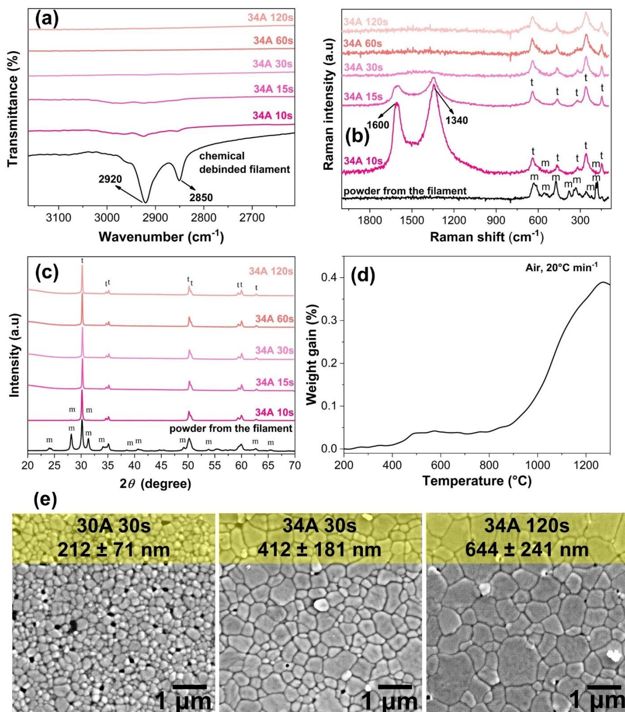
Figure 12: (a) Fourier Transform Infrared Spectroscopy (FTIR), (b) Raman, (c) X-ray diffraction (XRD) spectra of chemically debinded sample (1h in acetone) subjected to UHS under 34 A for different dwell times; the peaks of tetragonal and monoclinic zirconia are indexed as t and m , respectively. (d) TGA analysis of a UHS sample (26 A, 120 s) in air; (e) SEM micrographs showing the evolution of the microstructure with current and holding time.
