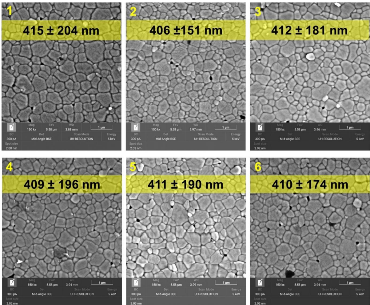
Figure 13: Microstructural analysis (after UHS at 34 A for 30 s) of different regions on the sample surface. The microstructures refer to samples chemically debinded for 1h in acetone before UHS.
