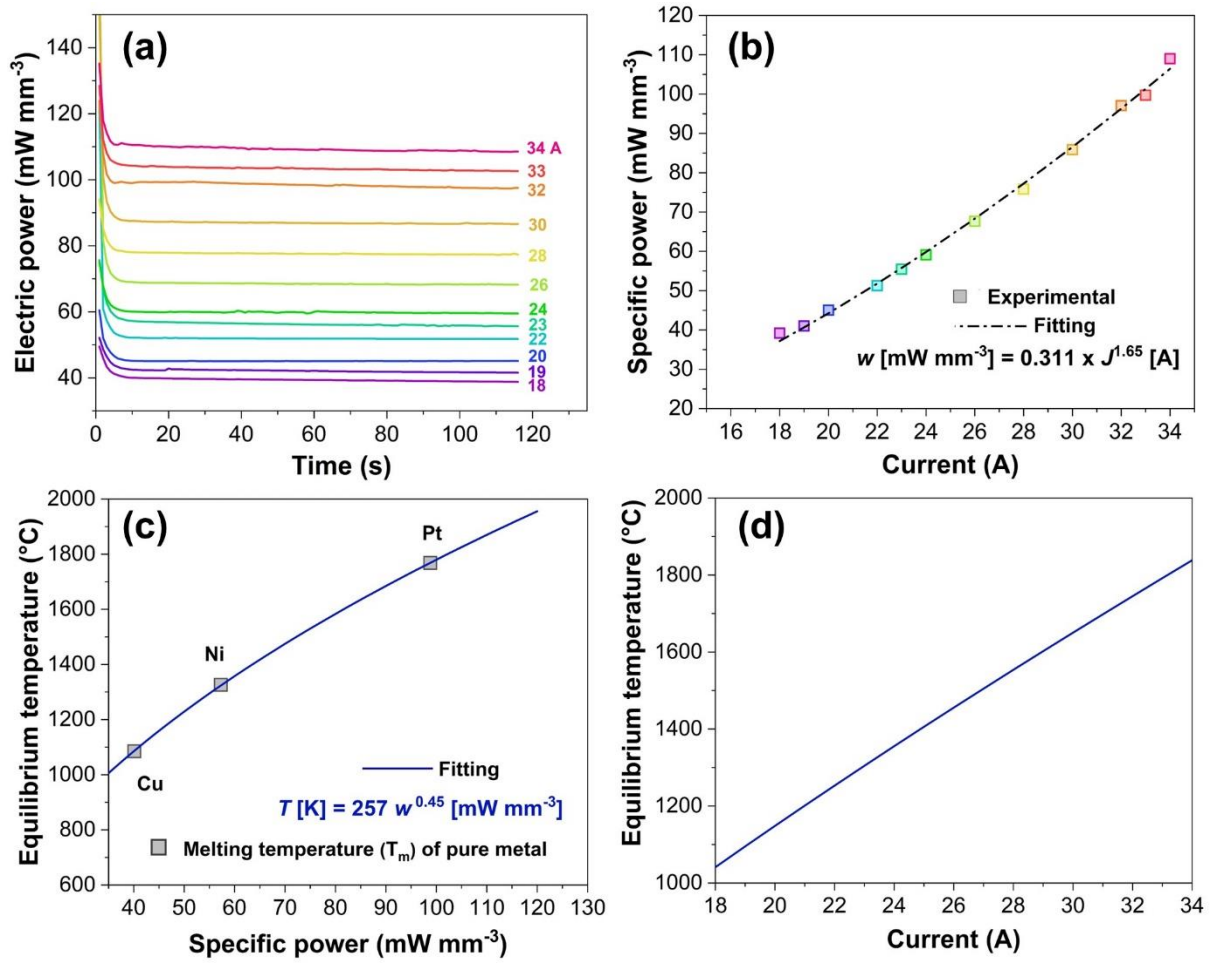
Figure 7: (a) Variation of the electric power of the felt as a function of time. (b) Maximum electrical power dissipated in the carbon felt as a function of the pre-set current (measured experimental values and fitting curve). (c) Equilibrium felt temperature as a function of power dissipated in the felt; fitting was performed on the experimental values identified with the help of pure metals having defined T_m ; for Ni, the Ni-C eutectic point at 1326 °C was selected as opposed to its melting temperature of 1455 °C. (d) Equilibrium felt temperature as a function of the applied electric current.
