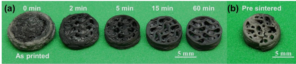
Figure 5: Optical image of the UHSed (a) chemically debinded samples at different soaking times in acetone at 40 °C. (b) pre-sintered sample. UHS experiments was carried out at 26A for 120s.
