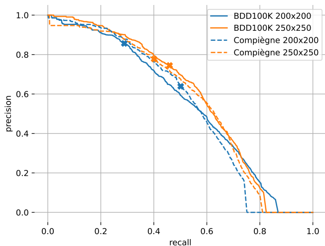
Fig. 7: Precision-Recall curves obtained after 100 epochs of training with BDD100K and Compiègne models with 200x200 and 250x250 box sizes. The points corresponding to precision-recall values obtained using a confidence threshold of 0.25 are visible using crosses.
