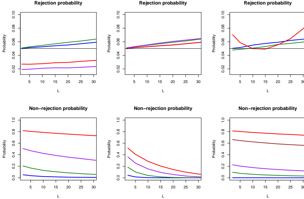
Figure 3: Empirical type-I (top panels) and type-II (bottom panels) errors obtained for 10,000 replications, shown as functions of L . Top row, left and middle displays: Example ( \mathcal{F}_1 ) with \xi = 0.25 (left) and 1 (middle). The underlying distribution is a Burr with \rho = -1 (blue), Fréchet (green), GPD (red) and Student (purple) distribution. Top row, right display: Example ( \mathcal{F}_2 ) with \rho = -5 (blue), -1 (green) and -0.5 (red). Bottom row, left display: Example ( \mathcal{F}_3 ) where the shape parameters are 0.25 vs 0.275 (red), 0.25 vs 0.3 (purple), 0.25 vs 0.325 (green) and 0.25 vs 0.35 (blue). Bottom row, middle display: Example ( \mathcal{F}_4 ) with \xi = 0.25 (blue), 0.5 (green), 0.75 (purple) and 1 (red). Bottom row, right display: Example ( \mathcal{F}_5 ), where the degrees of freedom are 2 vs 1 (blue), 2 vs 4 (green), 2 vs 4/3 (purple), 10/6 vs 4/3 (brown) and 2 vs 10/6 (red).
