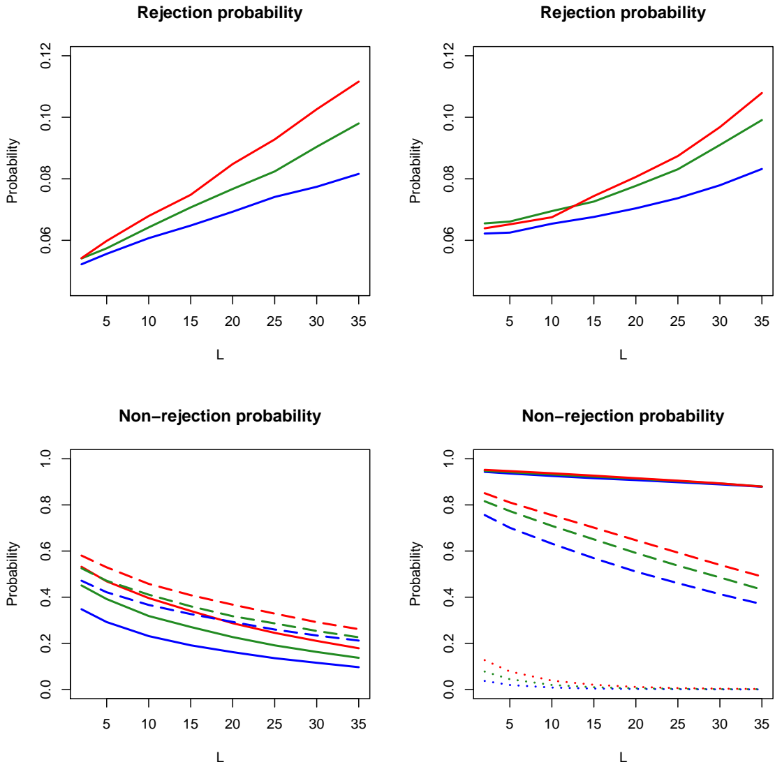
Figure 7: From left to right, top to bottom: examples (\mathcal{MF}) , (\mathcal{MM}) , (\mathcal{MP}) with \theta = 0.8 (solid curves) and \theta = 1.2 (dashed curves), and (\mathcal{CP}) with \pi = 0.2 (dotted curves), \pi = 0.5 (dashed curves) and \pi = 0.8 (solid curves). In all examples, n = 1,000 , \beta_n = 0.9 and J = 5 (blue curves), J = 10 (green curves) and J = 15 (red curves).
