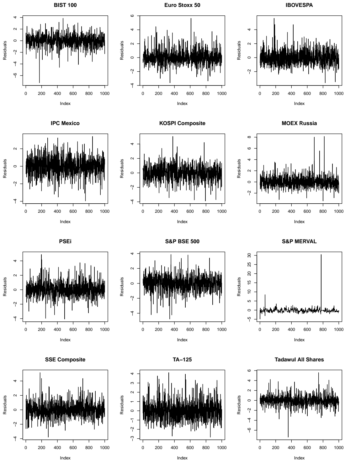
Figure 8: n = 1,000 ARMA(1,1)-GARCH(1,1) residuals associated with J = 12 times series of negative daily log-returns of stock market indices.
