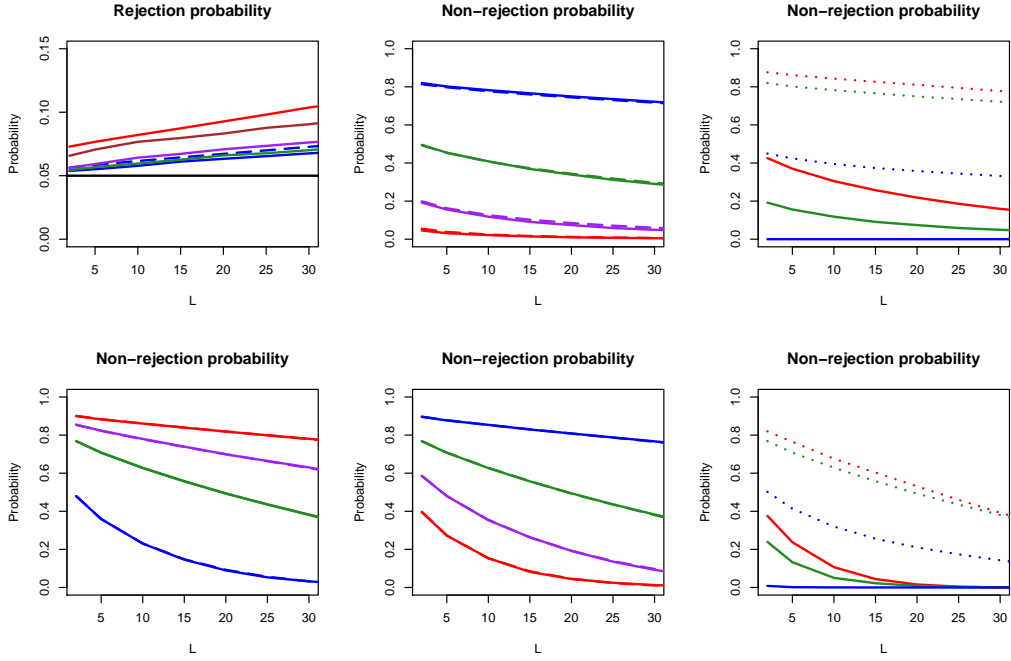
Figure 2: Empirical (solid curves) and approximated (dashed curves) type I (top left panel) and type II (other panels) errors obtained for 10,000 replications, as shown as functions of L . Top left: Example (\mathcal{P}) with \xi = 0.25 and: n_1 = n_2 = 1,000 (blue), n_1 = 1.5n_2 = 1,200 (green), n_1 \approx 2n_2 = 1,333 (purple), n_1 = 3n_2 = 1,500 (brown) and n_1 = 4n_2 = 1,600 (red). Top middle: Example (\mathcal{P}_\theta) with \xi = 0.25 and \theta_n = 1.1 (green curves), \theta_n = 1.2 (brown curves), \theta_n = 1.3 (blue curves) and \theta_n = 1.4 (red curves). Top right: same setting with a fixed \theta = 1.1 (dotted curves) or 1.3 (solid curves), and n = 500 (red), 1,000 (green) or 5,000 (blue). Bottom left: Example (\mathcal{P}_\lambda) with \lambda_n = 1.2 and \xi = 0.15 (blue curves), \xi = 0.25 (green curves), \xi = 0.35 (purple curves) and \xi = 0.5 (red curves). Bottom middle: same setting with \xi = 0.25 and \lambda_n = 1.1 (blue curves), \lambda_n = 1.2 (green curves), \lambda_n = 1.3 (purple curves) and \lambda_n = 1.4 (red curves). Bottom right: same setting with a fixed \lambda = 1.2 (dotted curves) or 1.5 (solid curves), and n = 500 (red), 1,000 (green) or 5,000 (blue). In all examples, n = 1,000 , \beta_n = 0.9 , \gamma = 0.05 and \alpha_{\ell,n} = 1 - \ell/n , \ell = 1, \dots, L .
