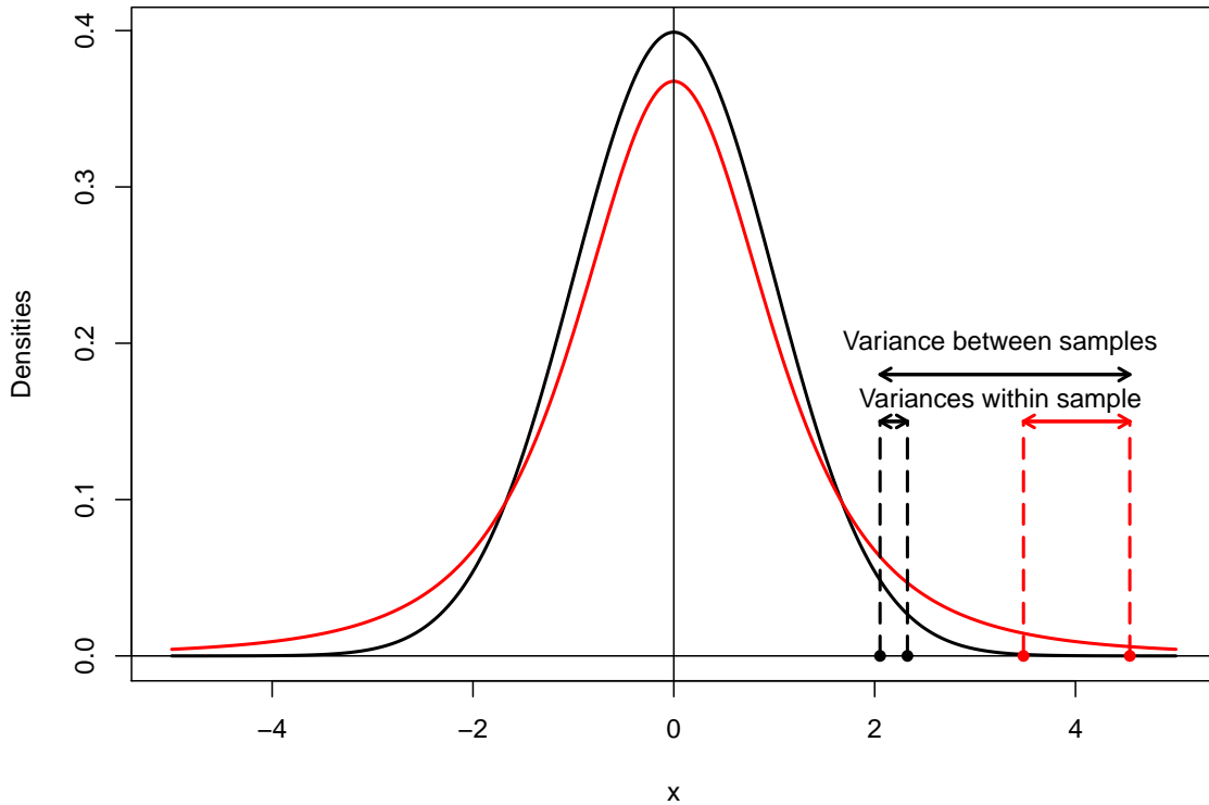
Figure 1: Decomposition of extreme log-quantile variance for a standard normal (black curve) and a Student's t distribution 3 degrees of freedom (red curve), for two extreme quantiles at probability levels \{0.98, 0.99\} .
