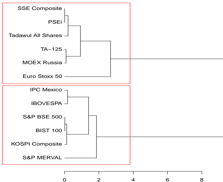
Figure 5: Dendrogram of 12 market stock indices, where the dissimilarity measure is the ANOVEX test statistic (and the linkage method is the complete-linkage) applied on their negative daily log-returns (pre-filtered by an ARMA(1,1)-GARCH(1,1) process).
