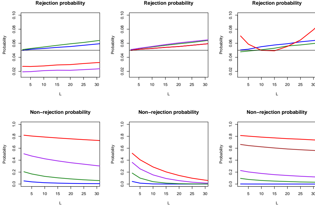
Figure 3: Empirical type-I (top panels) and type-II (bottom panels) errors obtained for 10,000 replications, shown as functions of L . Top row, left and middle displays: Example ( \mathcal{F}_1 ) with \xi = 0.25 (left) and 1 (middle). The underlying distribution is a Burr with \rho = -1 (blue), Fréchet (green), GPD (red) and Student (purple) distribution. Top row, right display: Example ( \mathcal{F}_2 ) with \rho = -5 (blue), -1 (green) and -0.5 (red). Bottom row, left display: Example ( \mathcal{F}_3 ) where the shape parameters are 0.25 vs 0.275 (red), 0.25 vs 0.3 (purple), 0.25 vs 0.325 (green) and 0.25 vs 0.35 (blue). Bottom row, middle display: Example ( \mathcal{F}_4 ) with \xi = 0.25 (blue), 0.5 (green), 0.75 (purple) and 1 (red). Bottom row, right display: Example ( \mathcal{F}_5 ), where the degrees of freedom are 2 vs 1 (blue), 2 vs 4 (green), 2 vs 4/3 (purple), 10/6 vs 4/3 (brown) and 2 vs 10/6 (red).
