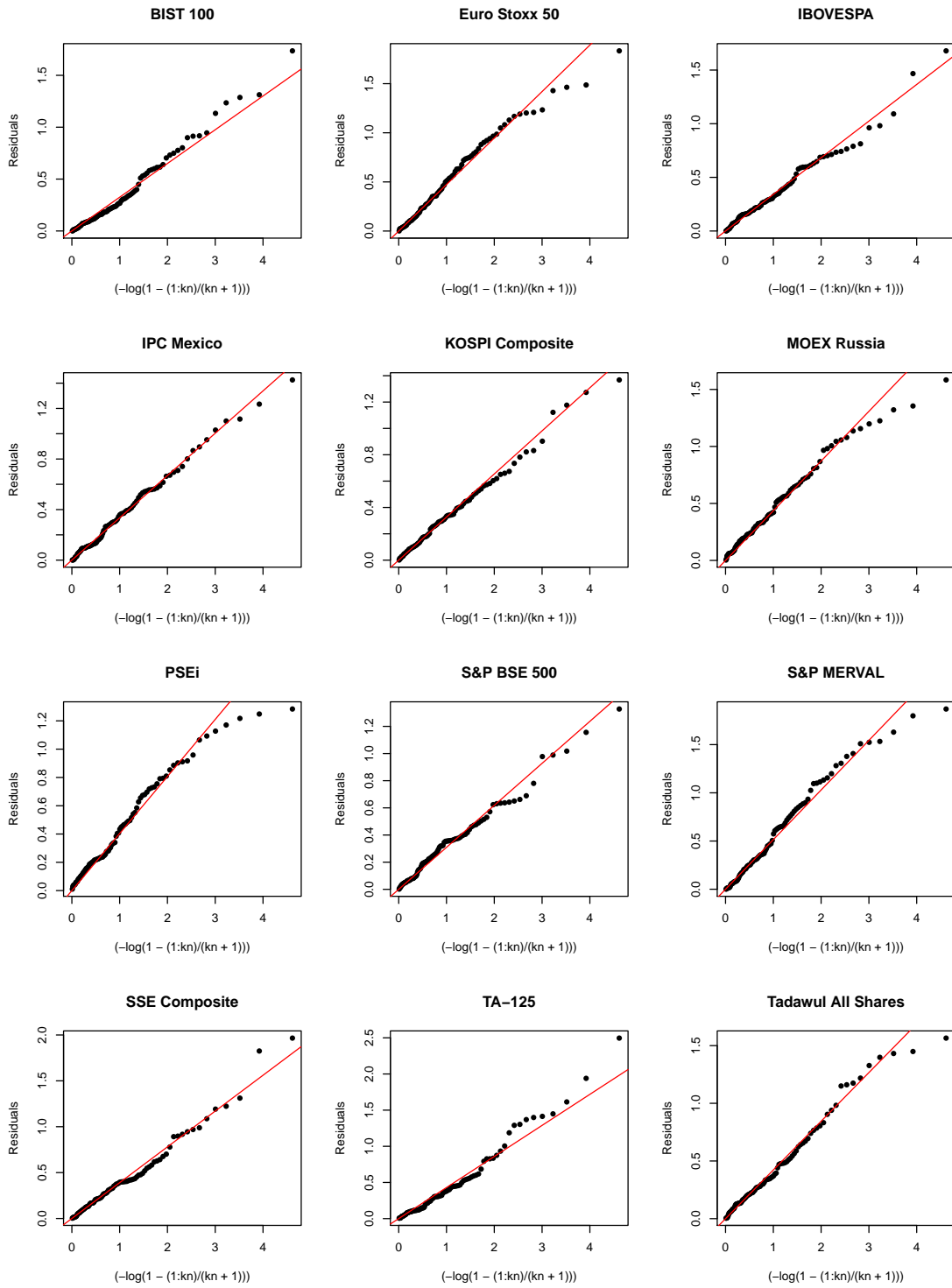
Figure 9: Exponential QQ-plots of the weighted log-spacings associated with the daily log-returns computed from 12 financial indices.
