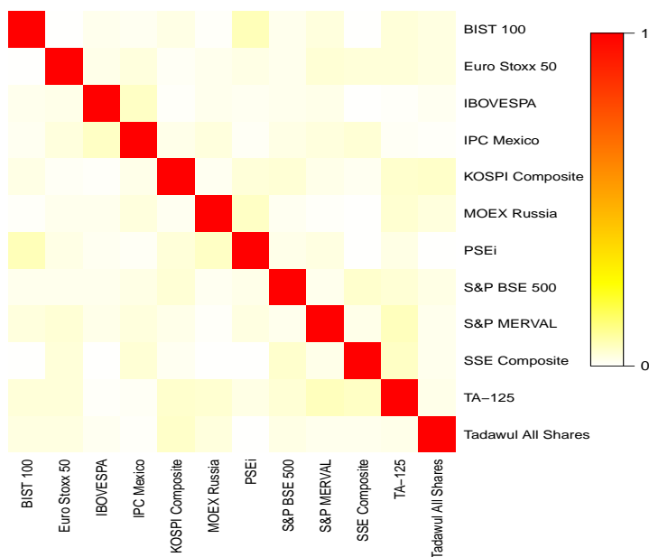
Figure 4: Correlation matrix (absolute values) between 12 series of negative daily log-returns of market stock indices (pre-filtered by an ARMA(1,1)-GARCH(1,1) process).
