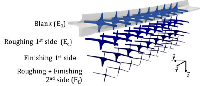
Figure 2. Geometric model of the cruciform, at each machining step.
