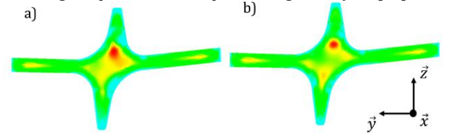
Figure 3. Reduced model of bulk RS field: (a) nominal RS field \mathbf{S}_n and (b) RS field prediction \mathbf{S}_r for a specific part, at an early stage of machining; with different RS field shapes, with traction (in yellow and red) in the core of the blank, and compression (in blue and green) close to the skin.
