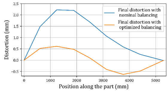
Figure 5. Reduction of final part distortion between nominal and optimized positioning in the blank, obtained by the DT behavior model.
