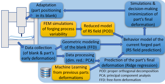
Figure 1. Hybrid digital twin of forged part, through bulk residual stress (RS) field, to reduce distortion in machining (online modules in bleu and offline ones in yellow).
