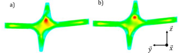
Figure 3. Reduced model of bulk RS field: (a) nominal RS field \mathbf{S}_n and (b) RS field prediction \mathbf{S}_r for a specific part, at an early stage of machining; with different RS field shapes, with traction (in yellow and red) in the core of the blank, and compression (in blue and green) close to the skin.
