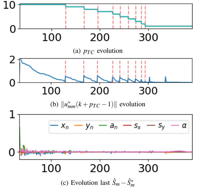
Fig. 6: Stability and convergence results
