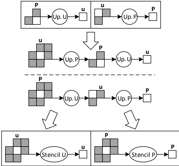
Fig. 3: Full stencil derivation for one iteration of \mathbf{u} and \mathbf{P} from the two initial half-stencils.
