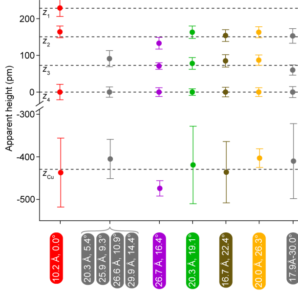
Figure 5: Average apparent heights ( z_{1-4} ) of fullerene molecules in the observed phases, and of the bare Cu(111) surface ( z_{Cu} ) around them. The bars visualize the statistical dispersion of the data.
