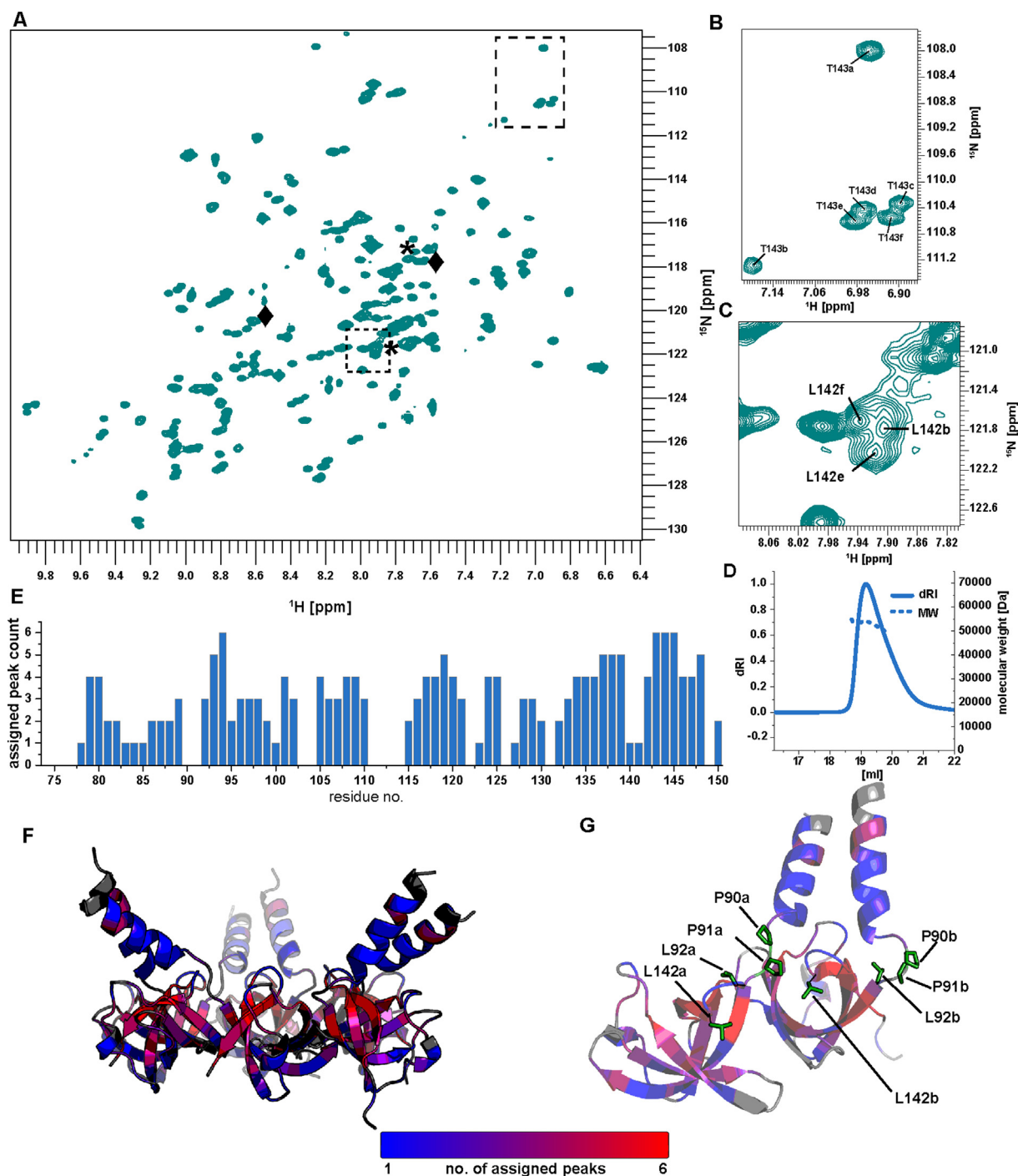
Figure 3. The PAN OB domain forms a hexameric complex. (A) ^1\text{H}, ^{15}\text{N} -TROSY spectrum of PAN 74-150 . The presence of 216 resolvable peaks reveals that PAN 74-150 exists in several different conformations. Sequential assignment yielded up to six peaks per residue. Diamonds and asterisks indicate the peak clusters corresponding to distinct conformations of L92 and L142, for which the three and four peaks, respectively, are located in very different regions of the spectrum. (B) and (C) Excerpts of the spectrum shown in A in dashed rectangles. (D) SEC-MALS analysis of PAN 74-150 , showing that the domain forms a hexamer of ~54 kDa. The dRI is reported on a relative scale from 0 to 1. The six conformations seen in (A) are likely to correspond to different conformations of the protomer in the hexameric complex. (E) Number of conformations identified and assigned for each residue. (F) Number of conformations assigned for each residue color-coded on the X-ray structure of PAN 74-150 OB domain (PDB entry 3H43). (G) Close-up of the structure in (F) highlighting the two different geometries of the P90–P91 amide bond ( cis and trans ) of the pair of neighbouring protomers whose N-terminal helices interact to form the coiled-coil structure. All spectra were recorded at 60 °C on an 850 MHz spectrometer with perdeuterated, ^{15}\text{N}, ^{13}\text{C} -labelled PAN 74-150 at 600 \mu\text{M} (monomer concentration).
