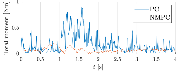
(f) Norm of the total moment at the CoM G generated by propellers with PC and NMPC.
