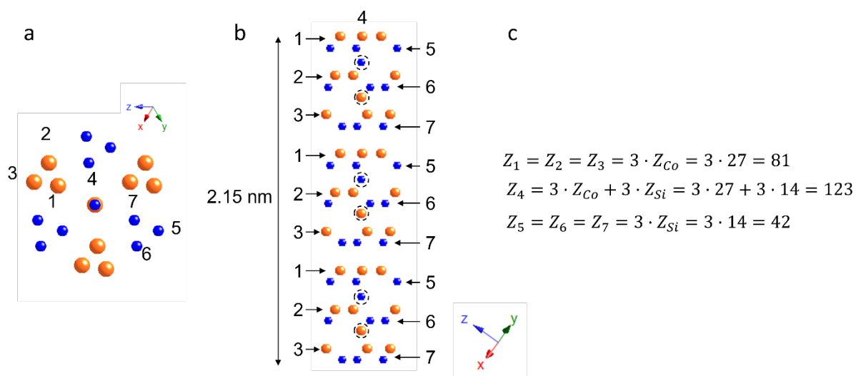
Figure S3. Schematic drawing of the CoSi structure along (a) the [1\bar{1}\bar{1}] direction and (b) the [110] direction perpendicular to [1\bar{1}\bar{1}] . (c) Cumulative atomic number of b atomic columns in a 2.15 nm-thick crystal.
