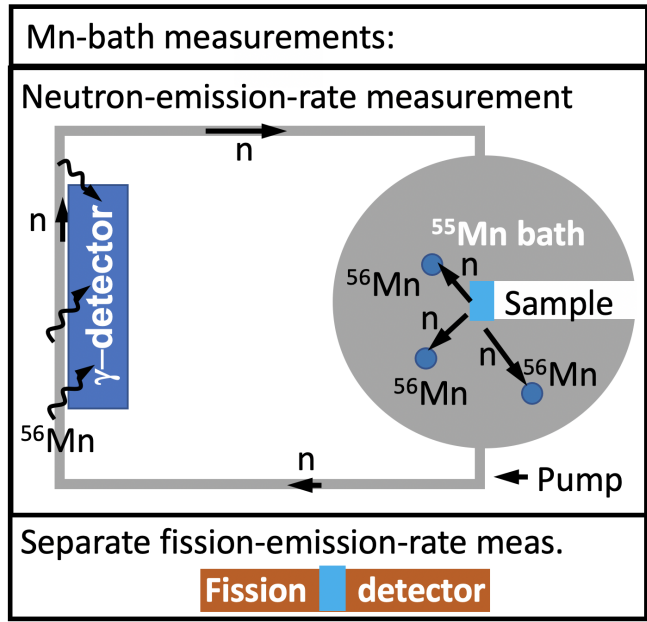
Figure 1: A schematic drawing of the absolute Mn-bath \bar{\nu}_f measurement type.
