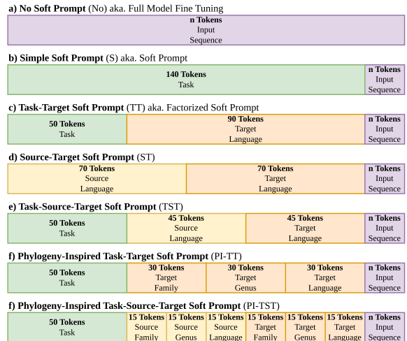
Figure 3: Composition of the input embeddings to the frozen model for different Soft Prompt variants.
