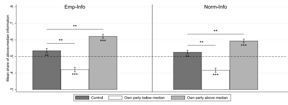
(b) Non-cheaters
