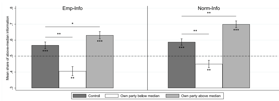
(c) Cheaters
