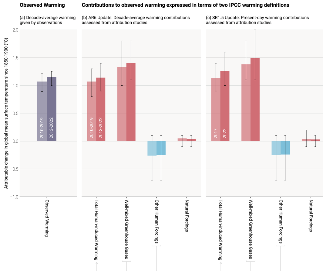
Figure 5. Updated assessed contributions to observed warming relative to 1850–1900; see AR6 WGI SPM.2. Results for all time periods in this figure are calculated using updated datasets and methods. The 2010–2019 decade-average -assessed results repeat the AR6 2010–2019 assessment, and the 2017 single-year -assessed results repeat the SR1.5 2017 assessment. For each double bar, the lighter and darker shading refers to the earlier and later period, respectively. The 2013–2022 decade-average and 2022 single-year results are the updated assessments for AR6 and SR1.5, respectively. Panel (a) shows updated observed global warming from Sect. 5, expressed as total GMST, due to both anthropogenic and natural influences. Whiskers give the very likely range. Panels (b) and (c) show updated assessed contributions to warming, expressed as global mean surface temperature, from natural forcings and total human-induced forcings, which in turn consist of contributions from well-mixed greenhouse gases and other human forcings. Whiskers give the likely range.
