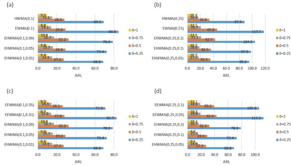
Pane 2: p = 3
