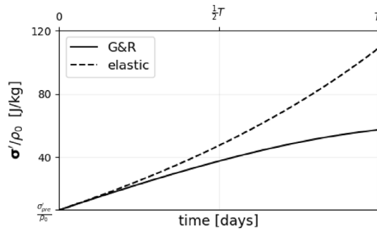
Fig. 8. Evolution of stress of the fiber pointing at the direction “ \mathbf{a}_1 ”, while being continuously pulled. The variable shown in the figure is “ \sigma' : (\mathbf{a}_1 \otimes \mathbf{a}_1) / \rho_0 ”. The solid line shows the stress configuration, if Eq. (37) is implemented. The dashed lines presented the same model, while assuming the constituents to behave elastically.
