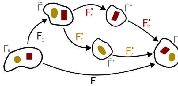
Fig. 1. Multiplicative split used in the Homogenized Constrained Mixture Theory and related configurations. We show an example of a mixture with 2 constituents: constituent “○” & constituent “□”.
