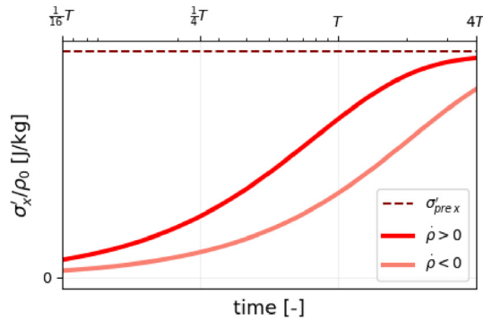
Fig. 6. Evolution of the Cauchy stress under a more pronounced deposition ( \dot{\rho}_0 > 0 ) and degradation ( \dot{\rho}_0 < 0 ).
