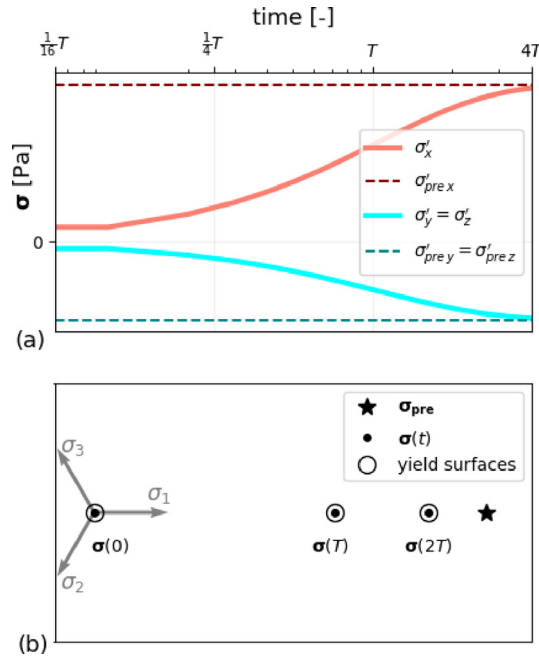
Fig. 4. (a) Evolution of the isochoric Cauchy stress components. (b) Stresses in the stress-space and viewed from the deviatoric plane.
