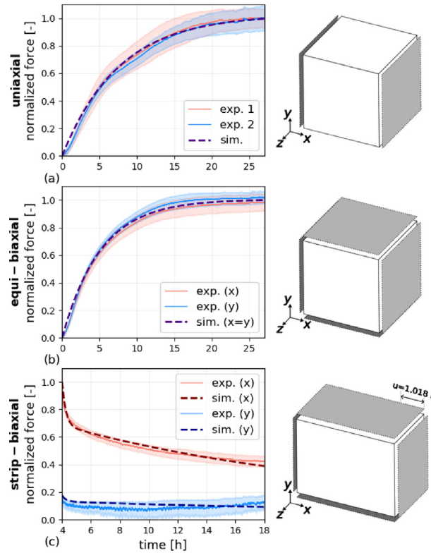
Fig. 5. (a) Measurements performed in a uniaxial setting. Eq. (31) was applied on a isotropic material with 2 mass turnover rates: T_1=7 hours ( \phi_1 = 50\% ) and T_2=8 hours ( \phi_2 = 50\% ). In order to reproduce the uniaxial protocol, \mathbf{F}_h was set to be \text{diag} \left[ \lambda, \frac{1}{\sqrt{\lambda}}, \frac{1}{\sqrt{\lambda}} \right] . (b) Measurements of the equi-biaxial setting. A single mass turnover rate of T=5 h was sufficient to fit our simulated data to the experiments. Here, \mathbf{F}_h was set to be \text{diag} \left[ \lambda, \lambda, \frac{1}{\lambda^2} \right] . (c) Strip-biaxial protocol after applying an initial stretch of \lambda_i = 1.018 to the cell-seeded collagen. A short mass turnover rate of T_1=0.21 h ( \phi_1 = 33\% ) and another of T_2 = 21 hours ( \phi = 67\% ) provided us with the simulated data shown in the graph. \mathbf{F}_h was set to be the same as in (b). Eichinger et al. [29] authorized the authors to expose their experimental data in this work.
