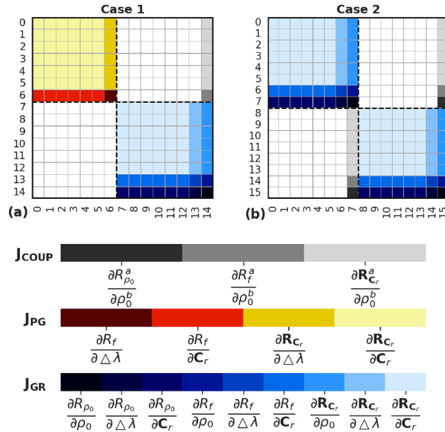
Fig. 2. Graphical illustration of the global Jacobian matrices of “case 1” [Eq. (36)] and “case 2” [Eq. (37)].
