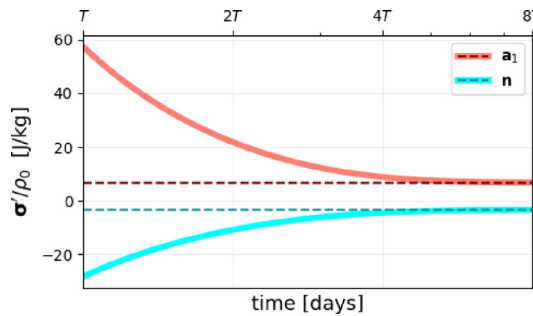
Fig. 9. Solid lines: Evolution of the stress components “ \sigma' : (\mathbf{a}_1 \otimes \mathbf{a}_1) / \rho_0 ” (red) and “ \sigma' : (\mathbf{n} \otimes \mathbf{n}) / \rho_0 ” (blue). Dashed lines: homeostatic targets “ \sigma'_{pre} : (\mathbf{a}_1 \otimes \mathbf{a}_1) / \rho_0 ” (red) and “ \sigma'_{pre} : (\mathbf{n} \otimes \mathbf{n}) / \rho_0 ” (blue). (For interpretation of the references to color in this figure legend, the reader is referred to the web version of this article.)
