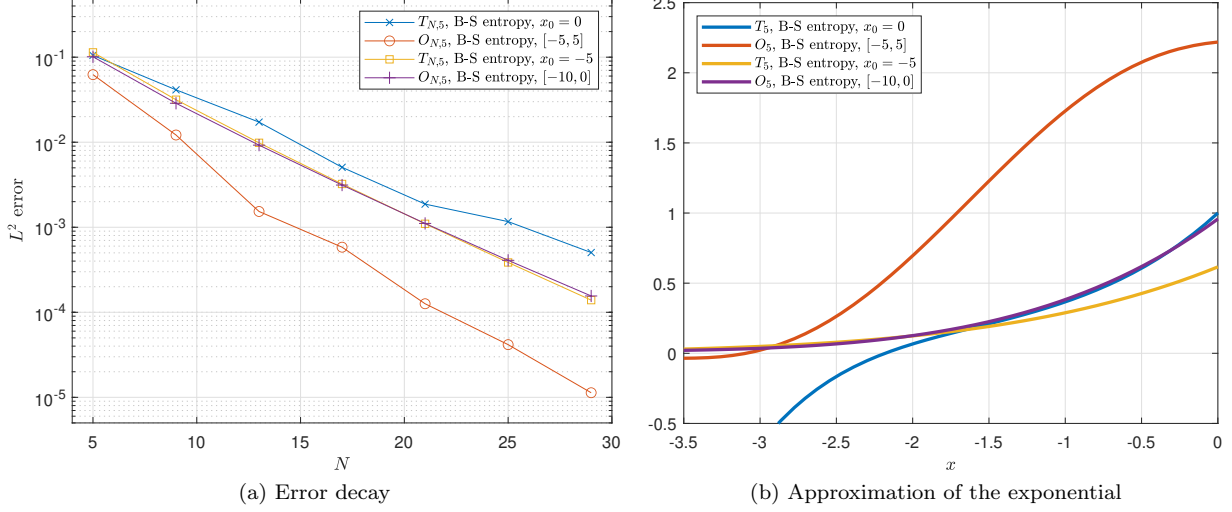
Figure 16: Error decay for approximations of the six-Gaussian function based on the Boltzmann-Shannon entropy and the corresponding approximations of the exponential function
