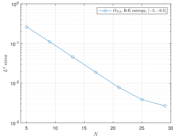
Figure 18: Error decay for approximations of the six-Gaussian function based on the Bose-Einstein entropy with matter.
