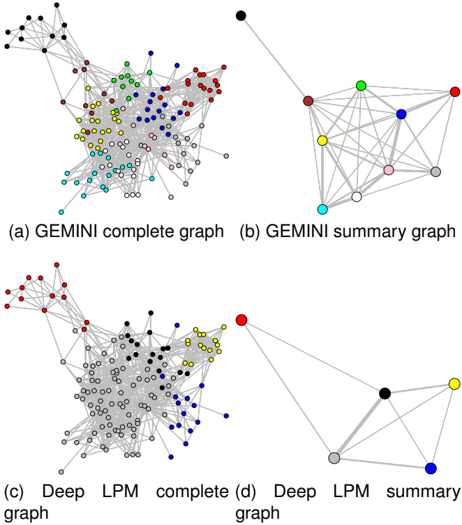
Fig. 8. Fruchterman Reingold representation of the Enron email interaction graph. Nodes are coloured according to clusters. The summary graph is a cluster-wise average of the positions of the nodes with edges as strong as the number of interactions between two clusters.
