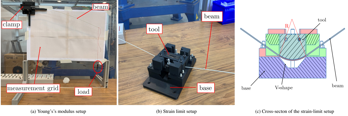
Figure 5: Experimental benchmarks. Figure (a) illustrates the Young's's modulus estimation setup, Figure (b) shows the strain limit estimation setup and Figure (c) gives details on the strain limit estimation setup.
