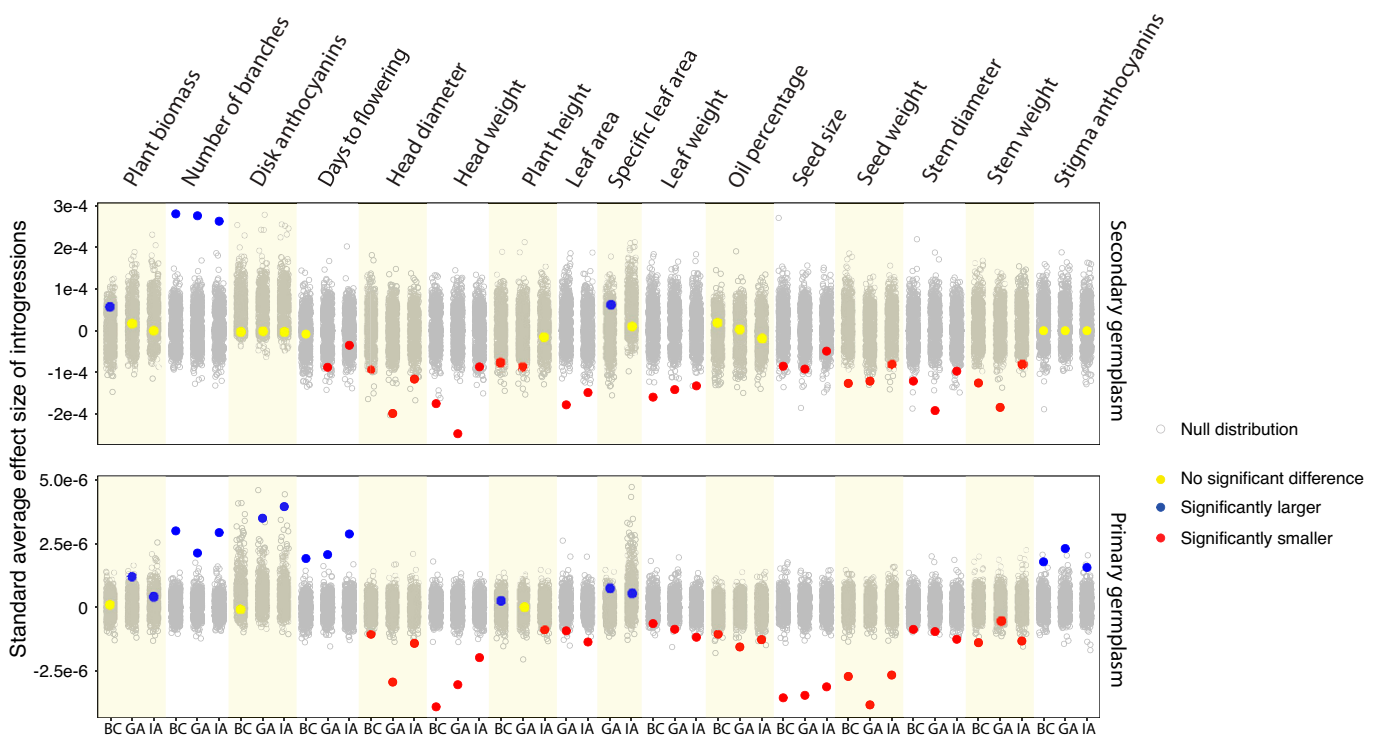
Fig. 5. Standardized average effect sizes of introgression variants from the ridge-regression BLUP model (calculated from Z-score-normalized trait values) in the SAM population. Gray dots show the null distribution of effect sizes. Red, blue, and yellow represent the decreasing, increasing, or neutral effects of introgressions on phenotypic traits at P value < 0.05 . BC, British Columbia; GA, Georgia; IA, Iowa.
