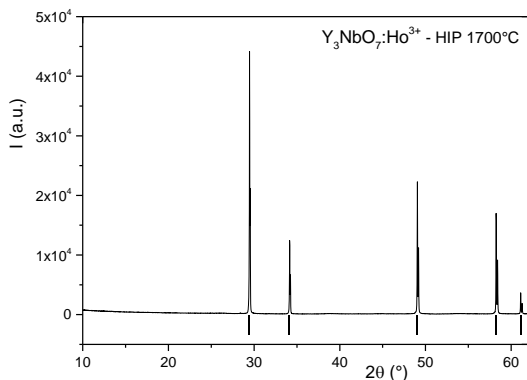
Figure 4- X-Ray diffraction pattern of the (1600°C-6hours, HIP 1700°C) pellet for which the lowest transmission is observed. This pattern confirms the absence of phase decomposition as all the peaks are attributed to the \text{Y}_3\text{NbO}_7 compound (indexation with the 00-036-1353 JCPDS file).
