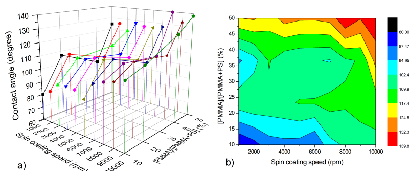
Figure 2: The dependence of the water contact angle on the polymer ratio \gamma_{pm} with \gamma_p = 5\% , spin-coating rotation speed v_s of samples in series A1.
