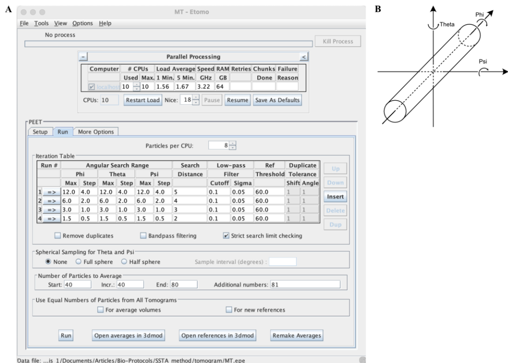
Figure 9. Configuration of the Run tab of Etomo. (A) Iteration runs. (B) Rotations used to adjust the subvolumes with the reference.
