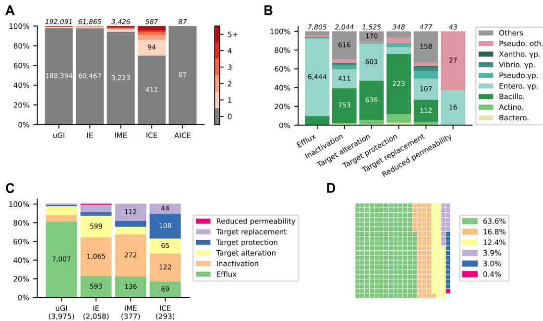
Figure 4. Diversity of antibiotic resistance mechanisms in cargo. (A) Distribution of GIs harbouring antibiotic resistance-related CDS per GI class. (B) Distribution of top-8 taxa per antibiotic resistance mechanism. (C) Distribution of antibiotic resistance mechanisms CDS count across GI classes. GIs containing multiple mechanisms are counted more than once. (D) Waffle chart of antibiotic resistance mechanisms distribution across all GIs bearing antibiotic resistance.
