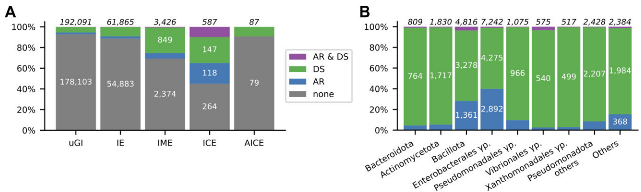
Figure 6. Coexisting antibiotic resistance mechanisms and defense systems in cargo. (A) Distribution of the absence or presence of at least one antibiotic resistance (AR) or defense system (DS) gene per GI class. (B) Distribution of AR, DS or both for each of the top-8 taxa.
