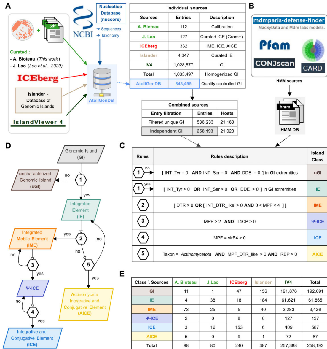
Figure 1. GI classification from AtollGenDB. (A) Number of raw entries for each of the five GI sources centralized in AtollGenDB. Quality control is performed on the total number of GIs to obtain AtollGenDB data to be analyzed, completed by sequence and taxonomy information from the NCBI Nucleotide database (nuccore). The number of unique and independent islands are then extracted. (B) HMM signature sources used for the classification and characterization steps. (C) Description of the five classification rules. (D) Description of the classification decision tree. (E) Classification results of the 258193 independent GIs by source.
