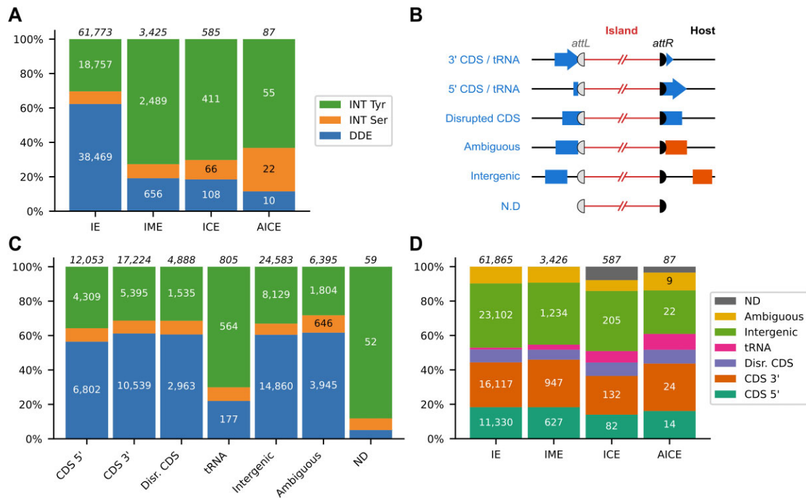
Figure 3. Integration modules and insertion sites characterization. (A) Distribution of integrase types across the various GI classes. The few GIs (95) containing more than one integrase type in the same CDS are not shown in the bars. (B) Illustration of the insertion site categories (see Material and Methods for definitions). Black hemispheres correspond to GI boundaries. (C) Distribution of integrase types across insertion sites. (D) Distribution of insertion sites across GI classes.
