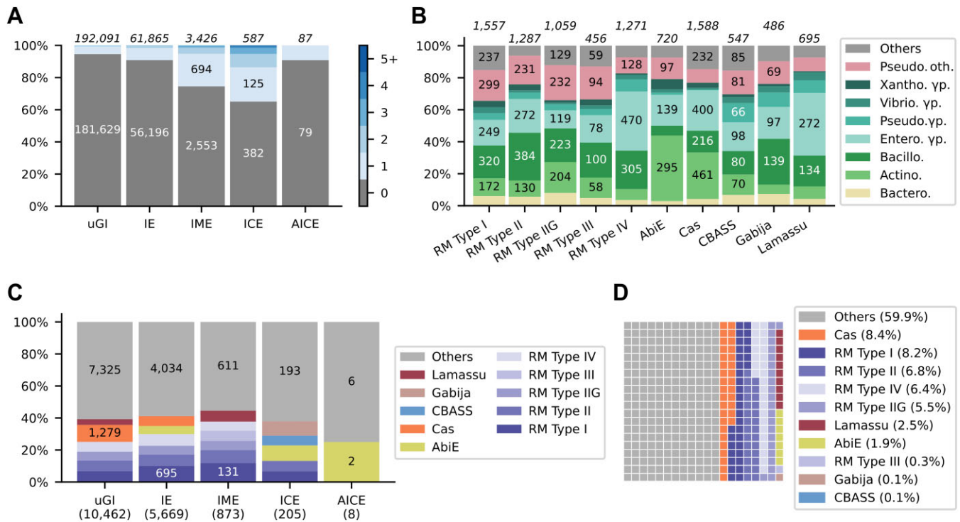
Figure 5. Diversity of defense systems in cargo. (A) Distribution of distinct and complete defense systems found per GI class. (B) Distribution of top-8 taxa across the top-10 defense systems found in data. (C) Distribution of the top-6 defense systems found in each GI class. (D) Waffle chart of the top-10 defense system distribution.
