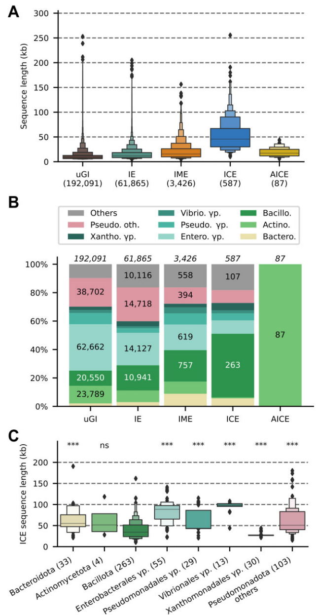
Figure 2. Sequence length and inter-taxa distributions. (A) Sequence length distribution of independent GIs across classes (total numbers in parenthesis). Two data points from the GI class exceeding 300 kb are not shown. (B) Distribution of top-8 taxa per GI class. (C) Sequence length distribution of ICEs across top-8 taxa. Statistical significance was calculated using Welch's t -test and the Bacillota phylum data as the reference (ns = not significant; *** P < 0.001).
