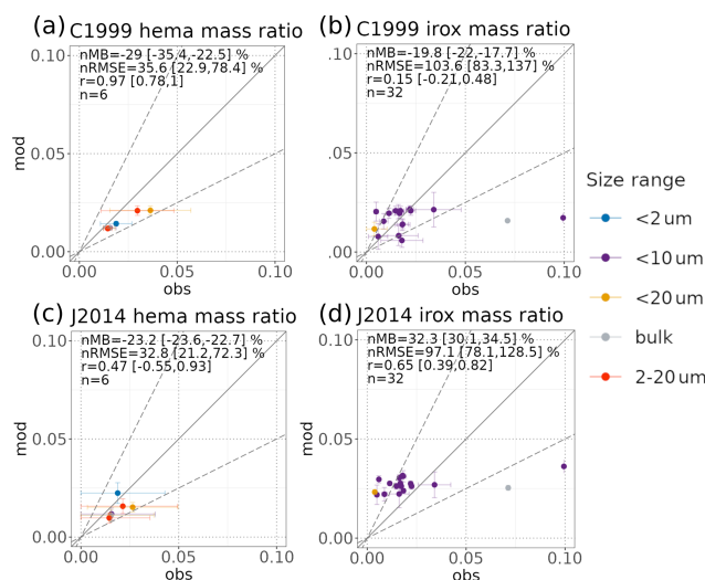
Figure 11. Comparison of the hematite – hema – and total iron oxides – irox – modeled versus observed mass fractions in the C1999 (a, b, respectively) and J2014 (c, d, respectively) experiments. Colors identify size ranges, circles correspond to observation points that fall within source regions as depicted in Fig. 2b, and triangles correspond to those outside. Statistics considering mean values are computed for all points within the modeled size ranges (up to 20\mu\text{m} in diameter). The ranges for the nMB, nRMSE and r correspond to the 95 % confidence level (see Sect. S1 for details).
