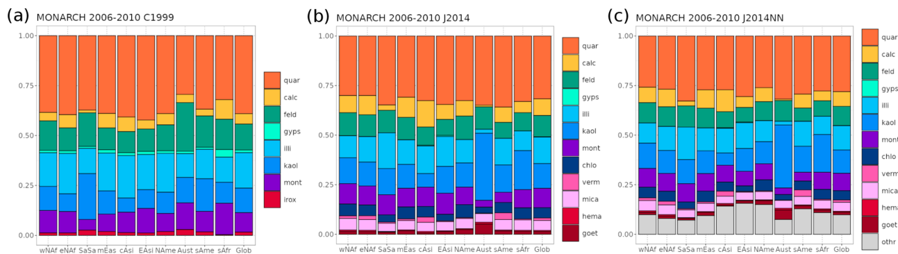
Figure 5. Mineral mass fractions at emission per region (from left to right, wNAf: western North Africa; eNAf: eastern North Africa; SaSa: the southern Sahara and Sahel; mEas: the Middle East and the Horn of Africa; cAs: central Asia; EAsi: East Asia; NAmE: North America; Aust: Australia; sAmE: South America; sAfr: southern Africa, and Glob: global; see Fig. 2b) estimated by MONARCH C1999 (a), J2014 (b) and J2014NN (c) annual means over 2006–2010. Quar: quartz; calc: calcite; feld: feldspar; gyps: gypsum; illi: illite; kaol: kaolinite; smec: smectite; irox: iron oxide; chlo: chlorite; verm: vermiculite; mica: mica; hema: hematite; goet: goethite; othr: other.
