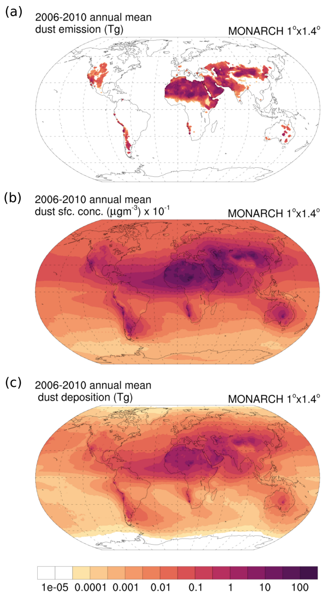
Figure 3. MONARCH-modeled homogeneous (a) dust annual mean emission (Tg), (b) surface concentration ( \mu\text{g m}^{-3} ) \times 10^{-1} and (c) total deposition (Tg), averaged over 2006–2010.
