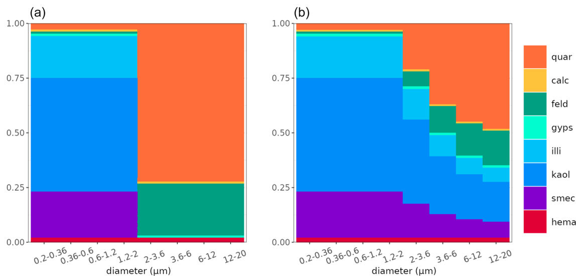
Figure 1. Normalized mass size distribution of minerals in the soil (a) and the aerosol (b) for the Xerosols Haplic soil type according to C1999-SMA. Quar: quartz; calc: calcite; feld: feldspars; gyps: gypsum; illi: illite; kaol: kaolinite; smec: smectite; hema: hematite.
