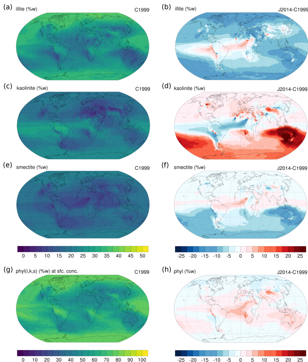
Figure 6. Annual mean (a) illite, (c) kaolinite and (e) smectite and the (g) sum of all clay mineral mass fractions (wt %) at surface concentration in C1999. Differences in annual mean (b) illite, (d) kaolinite, (f) smectite and (h) all clay mineral mass fractions (wt %) at surface concentration in J2014 with respect to C1999.
