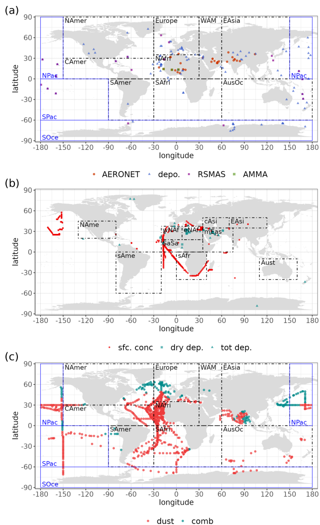
Figure 2. (a) Locations of the surface concentration (RSMAS, AMMA) and deposition (depo.) observations used for the dust evaluation and domains defined to compute regional statistics (in boxes). The 35 AERONET sites resulting from the filtering for dust events described in Sect. 4.3 are represented by red dots on the map. (b) Locations of the samples of mass mineral fractions in dust surface concentration (sfc. conc.) and dry (dry dep.) and total (tot. dep.) deposition used in this study. Source regions, as defined by Kok et al. (2021), considered for the regional analyses are depicted with boxes. (c) Locations of the total iron concentration measurements from Myriokefalitakis et al. (2018). Red dots correspond to those influenced by dust aerosols and used for evaluation purposes in this study.
