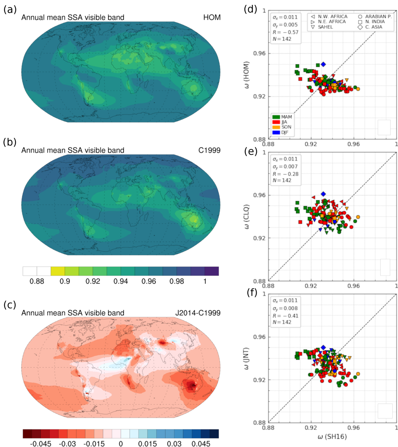
Figure 12. Annual mean single-scattering albedo (SSA), averaged in the UV-VIS band (0.3–0.77 \mu\text{m} ), considering dust to be an optically homogeneous species (a), as the sum of three optically different species using (b) C1999-modeled mineralogy. Differences between the latter and (c) J2014-modeled mineralogy. Comparison of monthly mean UV-VIS SSA, calculated considering dust to be a homogeneous species (d), and the mineralogy provided by C1999 (e) and J2014 (f) against dust-filtered SSA (averaged in the UV-VIS band) from AERONET version-3 level-2.0 Almucantar retrievals at the selected AERONET stations and months, labeled by region and season.
