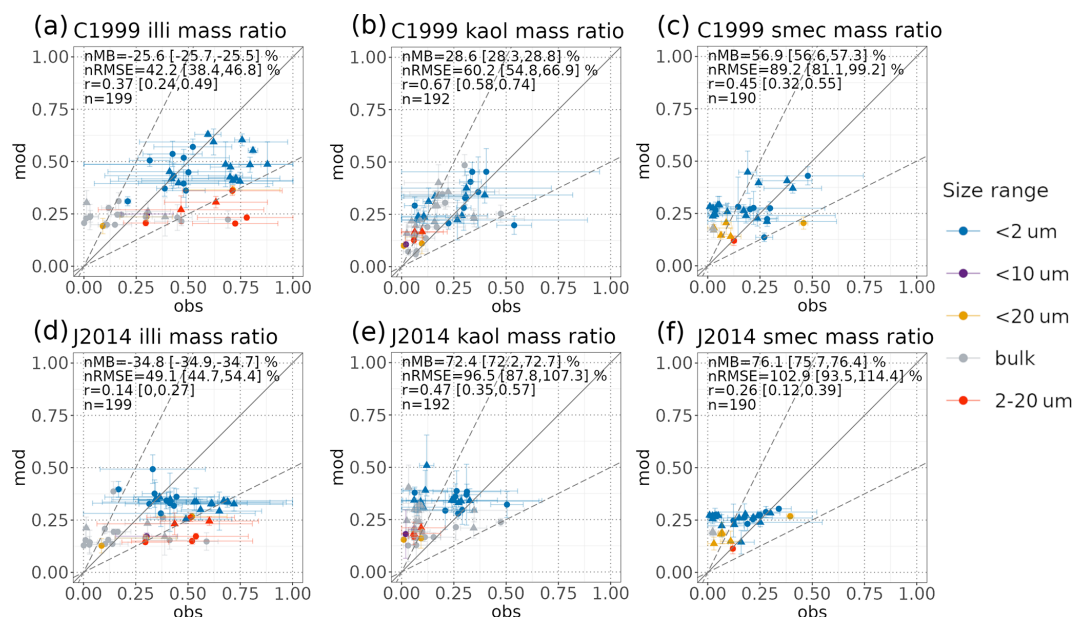
Figure 7. Comparison of the illite (illi), kaolinite (kaol) and smectite (smec) modeled vs. observed mass fractions in the C1999 (a–c, respectively) and J2014 (d–f, respectively) experiments. Colors identify size ranges, circles correspond to observation points that fall within source regions as depicted in Fig. 2b, and triangles correspond to those outside. Statistics considering mean values are computed for all points within the modeled size ranges (up to 20 \mu\text{m} in diameter). The ranges for the nMB, nRMSE and r correspond to the 95 % confidence level (see Sect. S1 for details).
