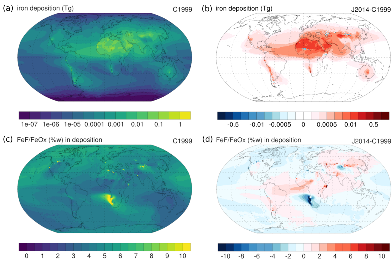
Figure 14. Total iron deposition and ratio of ferrihydrite and nano-iron oxides (FeF) over pure crystalline iron oxides (FeOx) according to C1999 (a, c, respectively). Differences compared to J2014 (b, d, respectively). The iron content of phyllosilicate minerals and feldspars is taken from Journet et al. (2014) and for hematite and goethite from Journet et al. (2008). FeF is calculated as the sum of the fast- and intermediate-dissolution iron pools in Ito and Shi (2016), i.e., 1.95 wt % (0.65 wt % and 1.3 wt %, respectively) of the total iron.
