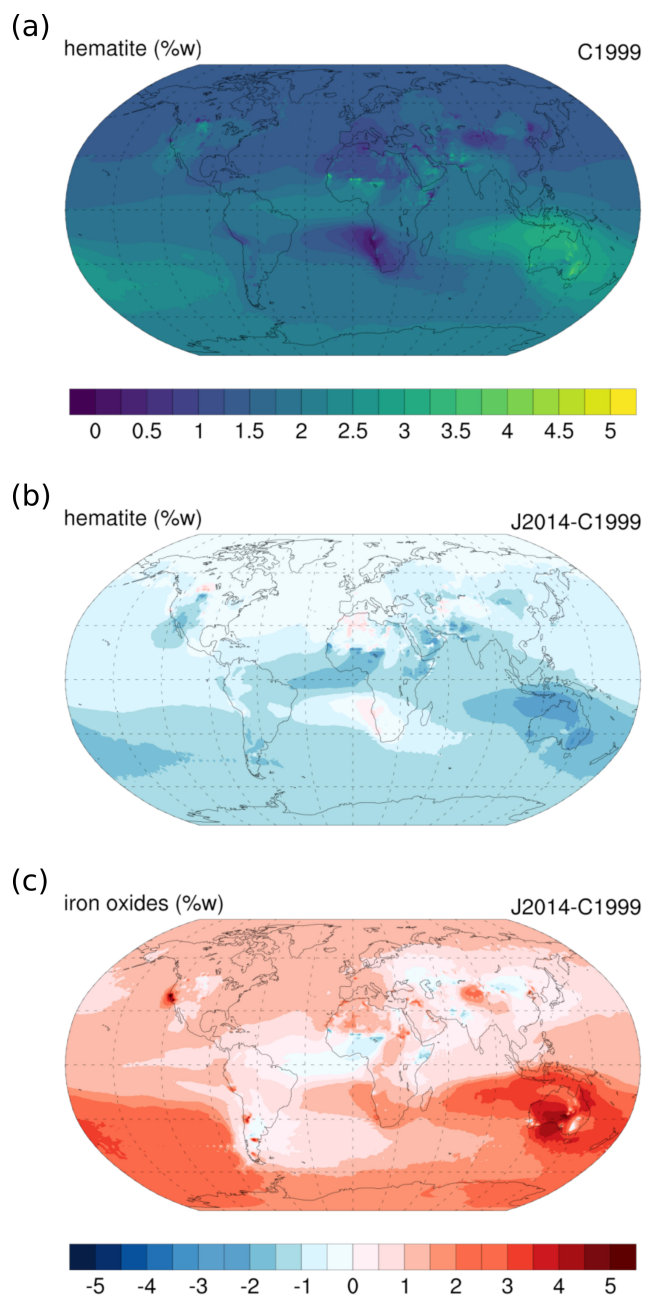
Figure 10. Annual mean hematite (iron oxide) mass fraction (wt %) in surface concentration in C1999 (a) and differences compared to hematite in J2014 (b) and to iron oxides (hematite plus goethite) in J2014 (c).
