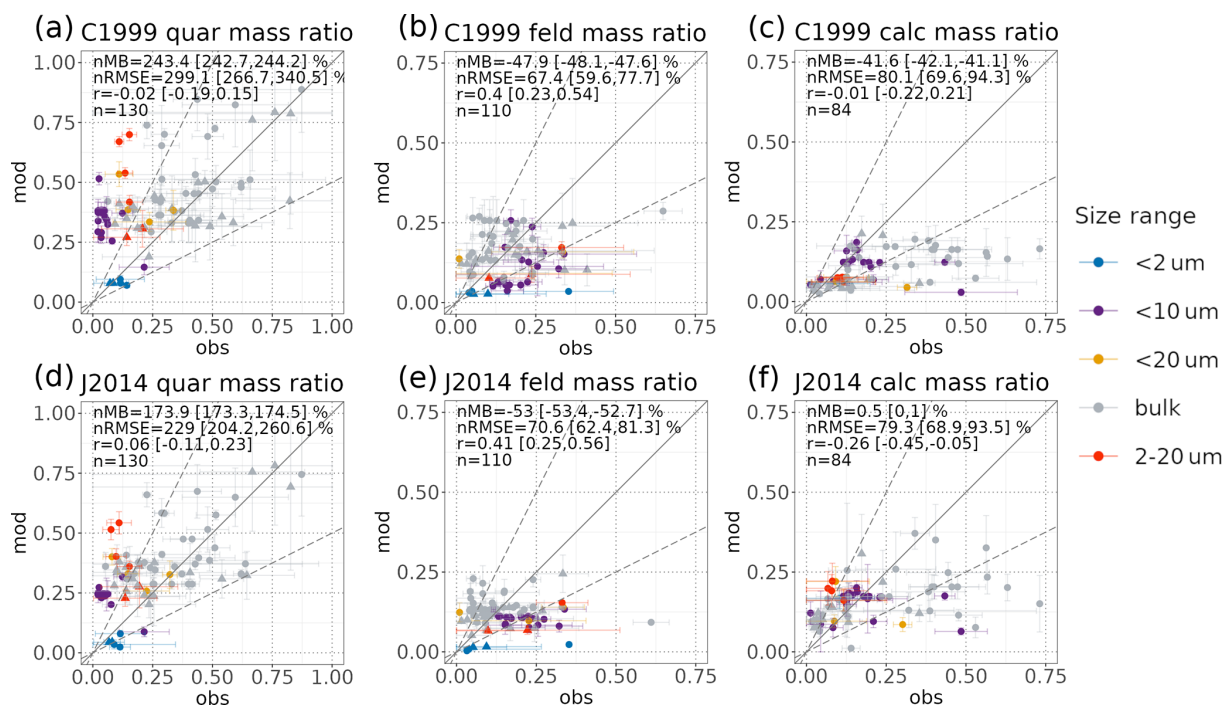
Figure 9. Comparison of the quartz, feldspar and calcite modeled vs. observed mass fractions in the C1999 (a–c, respectively) and J2014 (d–f, respectively) experiments. Colors identify size ranges, circles correspond to observation points that fall within the source regions as depicted in Fig. 2b, and triangles correspond to those outside. Statistics considering mean values are computed for all points within the modeled size ranges (up to 20 μm in diameter). The ranges for the nMB, nRMSE and r correspond to the 95 % confidence level (see Sect. S1 for details).
