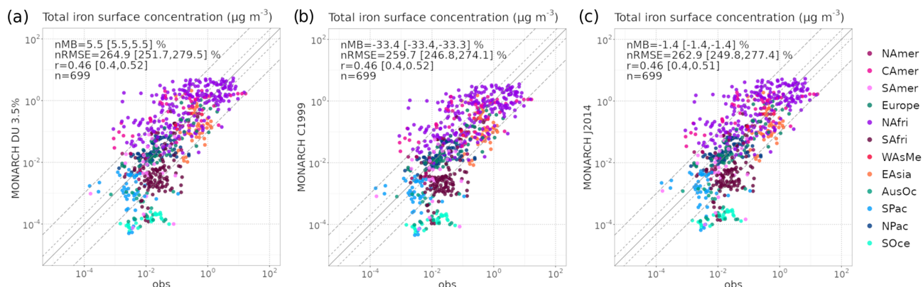
Figure 13. Diagnostic of the total iron surface concentration ( \mu\text{g m}^{-3} ) associated with the MONARCH-modeled (a) dust with an average of 3.5 wt % of iron content, (b) C1999 and (c) J2014 dust mineralogy compared with the observations compiled in Myriokefalitakis et al. (2018) identified as dust-dominated (see Fig. 1c and Sect. 4.4), where n is the number of measurements, nRMSE is the normalized root mean square error, nMB is the normalized mean bias, and r is the correlation over all the points. The ranges for the nMB, nRMSE and r correspond to the 95 % confidence level (see Sect. S1 for details). Regions are depicted in Fig. 1c. Dashed lines represent differences of 2 times and 1 order of magnitude.
