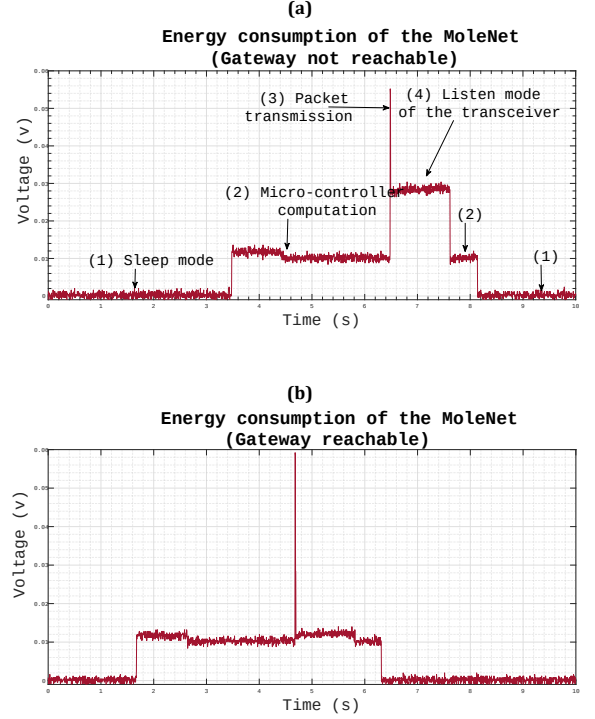
Fig. 8 – Energy consumption of the MoleNet during a round. (a) Energy consumed when the gateway is not reachable. (b) Energy consumed when the gateway is reachable.
