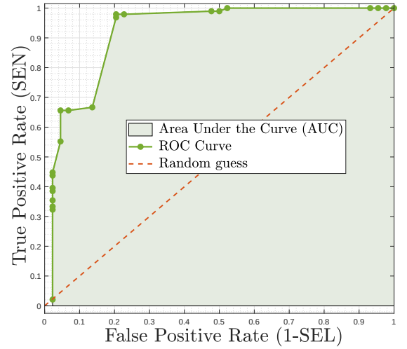
Evaluation of FuzDeMa performances (ROC Curve / AUC)
