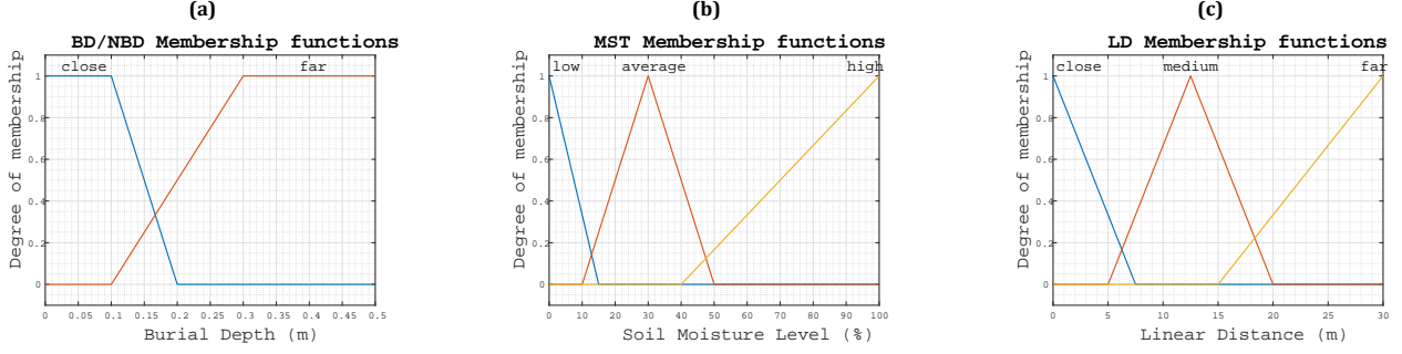
Fig. 3 – (a) Membership functions of the transmitter (BD) and receiver (NBD) burial depths. (b) Membership functions of the soil moisture level (MST). (c) Membership functions of the distance between the transmitter and the receiver (LD).
