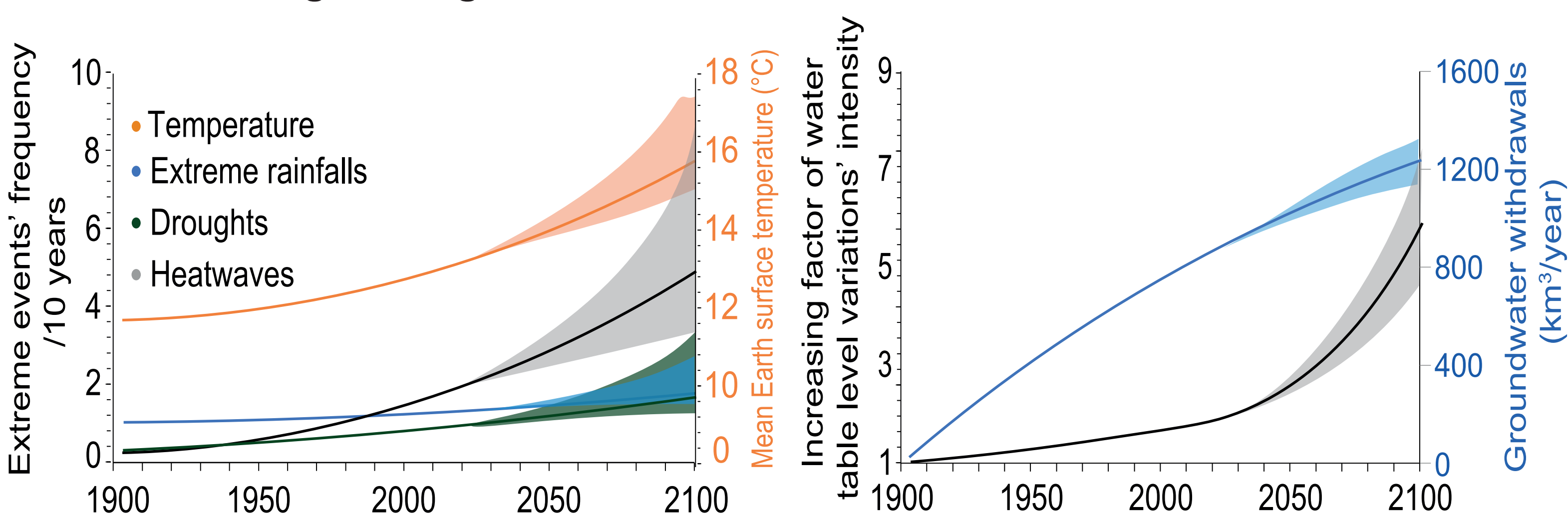
Fig.2. Measured and projected changes in average land surface temperature, intensity and frequency of extreme climate events, groundwater withdrawal and groundwater level variations' intensity from 1900 to 2100 (IPCC 2021; EEA 2021; Wada 2016).
