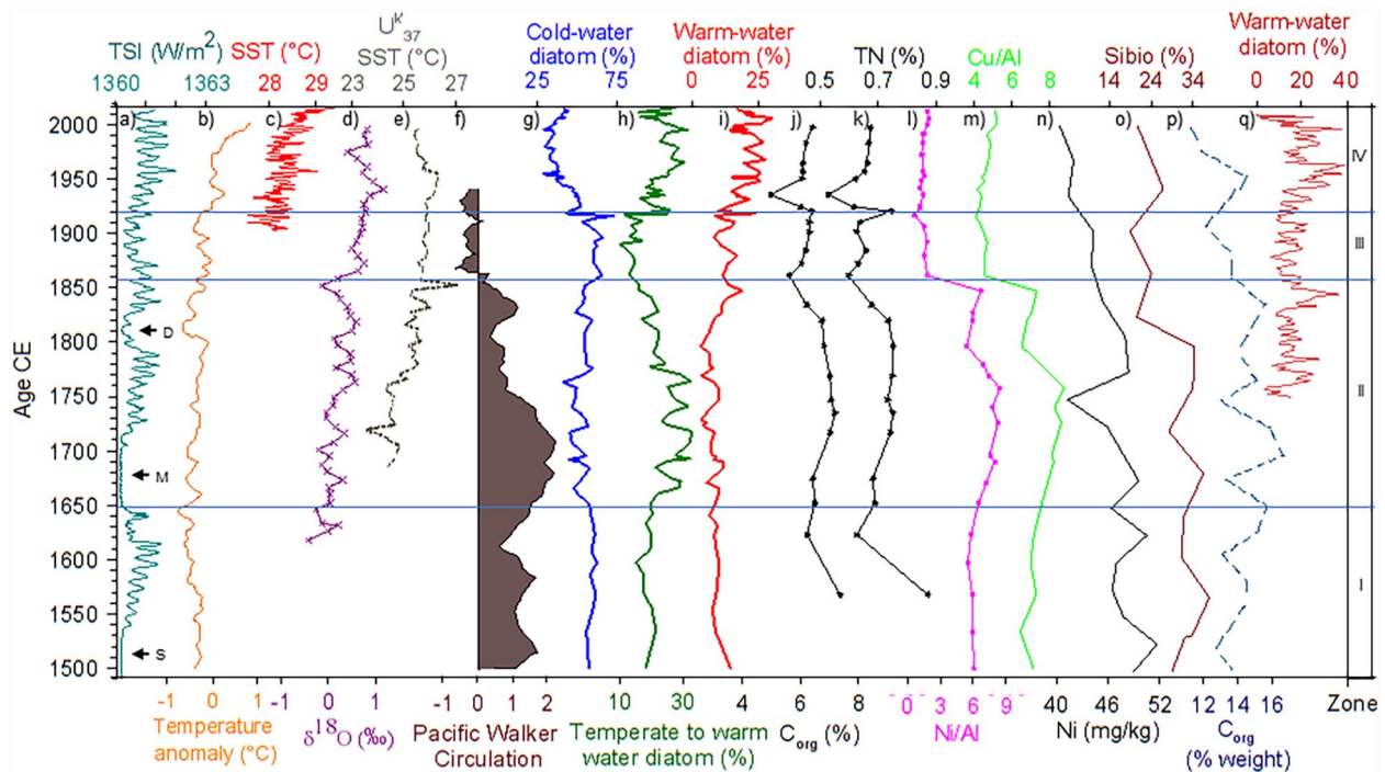
Figure 5. Paleoclimate records and the Tehua XII E03 record during the studied period. (a) Total Solar Irradiance (TSI, W/m^2 ), Spörer (S), Maunder (M) and Dalton (D) minima (Lean, 2018). (b) Surface temperature anomaly ( ^{\circ}C ) from the Northern Hemisphere (Mann et al., 2009). (c) SST ( ^{\circ}C ) from GoT (IRI, 2015). (d) stratification of the water column (Staines-Urías et al., 2009) from Gulf of California. (e) Alkenone-derived SST ( U^{k}_{37} ^{\circ}C ) from Guaymas Basin (Goni et al., 2006). (f) Pacific Walker Circulation strength (Griffiths et al., 2016). (g) Cold-water diatom (%), (h) temperate-water diatom (%), (i) warm-water diatom (%), (j) C_{org} (%), (k) TN (%), (l) Ni/Al, and (m) Cu/Al from GoT (this study). (n) Ni concentration (mg/kg) (Choumiline et al., 2019) and (o) biogenic silica (Sibio %) (Barron and Bukry, 2007) from Gulf of California. (p) C_{org} (weight %) from off the Baja California margin (Juárez et al., 2014). (q) Warm-water diatom from Santa Barbara Basin (Barron et al., 2013). Horizontal lines indicate the periods (I to IV) identified with CONISS analysis.
