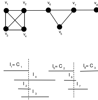
Fig. 2: An interval graph G and its interval representation \Gamma . We have, C_1 = I_1 , C_2 = I_5 and C_3 = I_8 , and hence \Gamma_1 = \{I_1, I_2, I_3, I_4\} , \Gamma_2 = \{I_5, I_6, I_7\} , \Gamma_3 = \{I_8\} .
