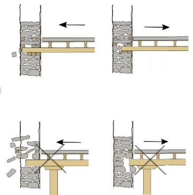
Connection of the wooden structure and the masonry walls , possible options– CRAterre©
