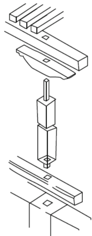
Flexible timber technology in Newari architecture – ©Toffin
