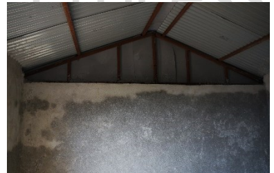
Finished house covered with CGI sheets on a metal structure, without ventilation, wall covered with cement plaster: indoor air condenses in the walls and roof. Cool materials radiate. Dhap, 2019—©CRAterre
